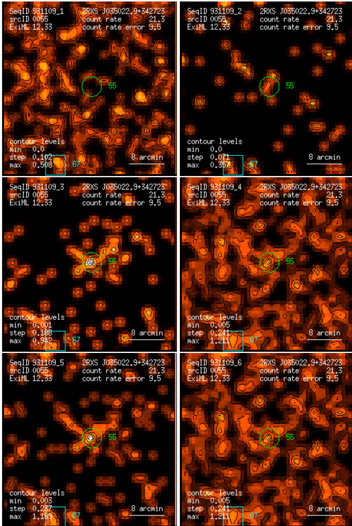
Figure 55: RASS 931109: detection 0055: band rate images, Gaussian filter: (1) PSPC channels 11 – 41, (2) 52 – 90, (3) 91 – 201, (4) 11 – 235, (5) 52 – 201, (6) 11 – 201. Broad band rates in counts/ks. Band rate contour levels in counts/ks/arcmin 2 .
