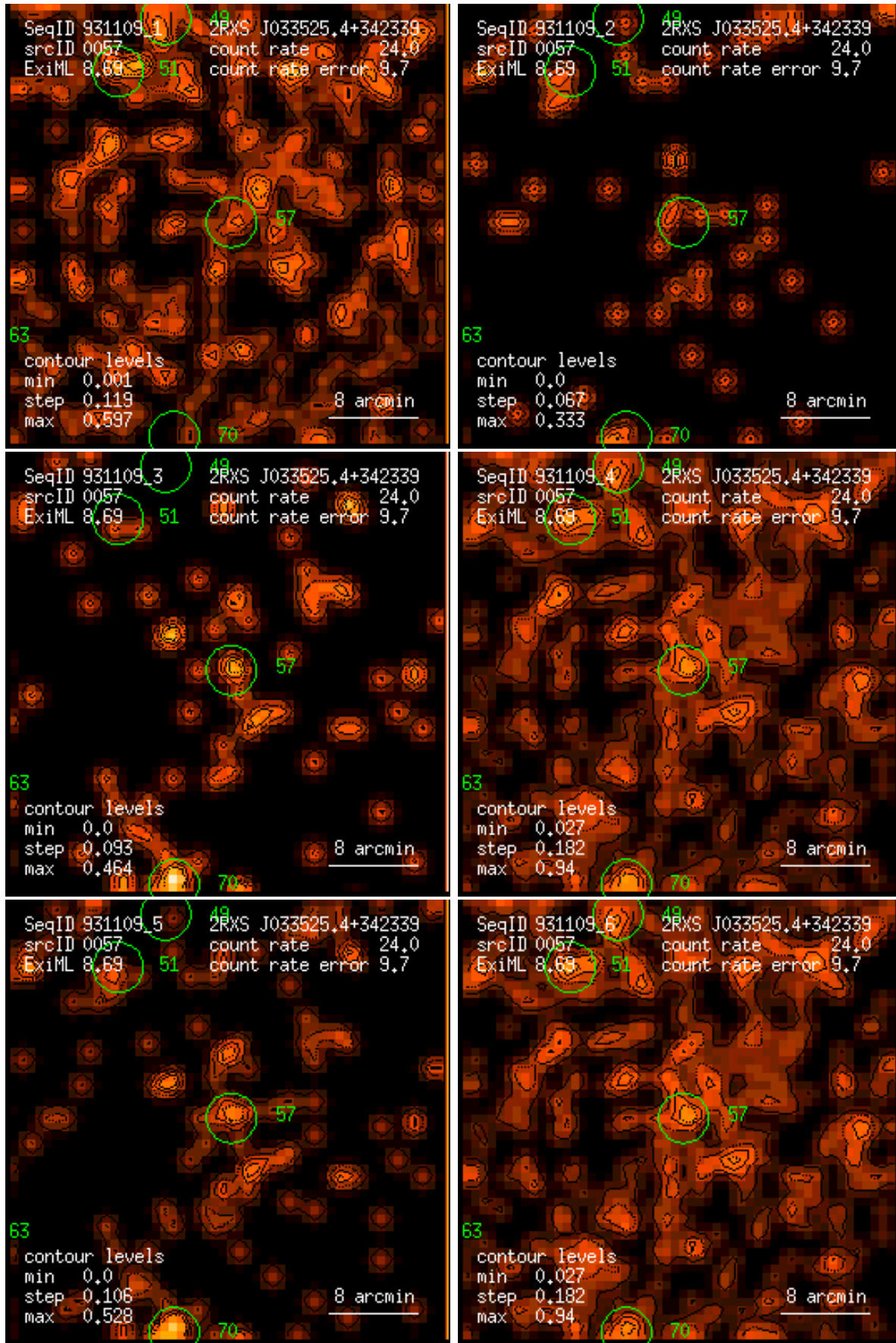
Figure 57: RASS 931109: detection 0057: band rate images, Gaussian filter: (1) PSPC channels 11 – 41, (2) 52 – 90, (3) 91 – 201, (4) 11 – 235, (5) 52 – 201, (6) 11 – 201. Broad band rates in counts/ks. Band rate contour levels in counts/ks/arcmin 2 .
