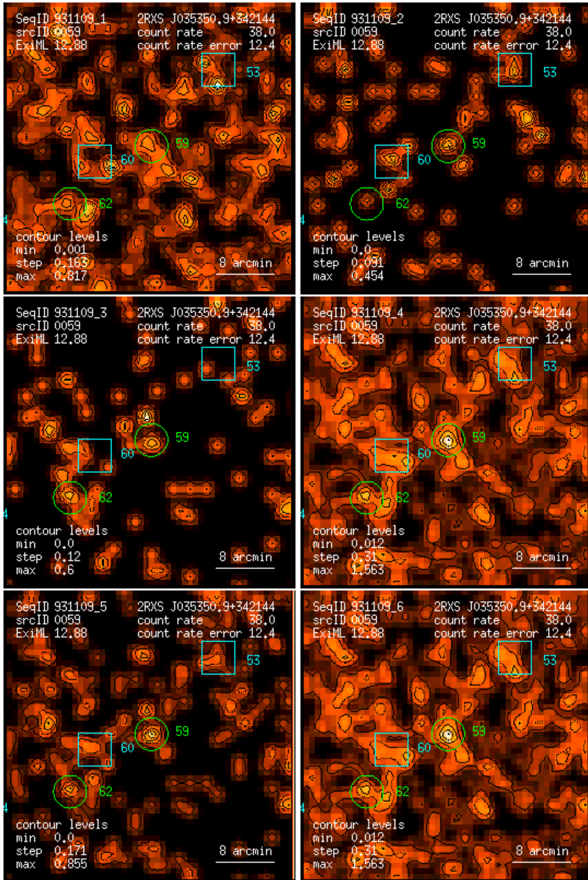
Figure 59: RASS 931109: detection 0059: band rate images, Gaussian filter: (1) PSPC channels 11 – 41, (2) 52 – 90, (3) 91 – 201, (4) 11 – 235, (5) 52 – 201, (6) 11 – 201. Broad band rates in counts/ks. Band rate contour levels in counts/ks/arcmin 2 .
