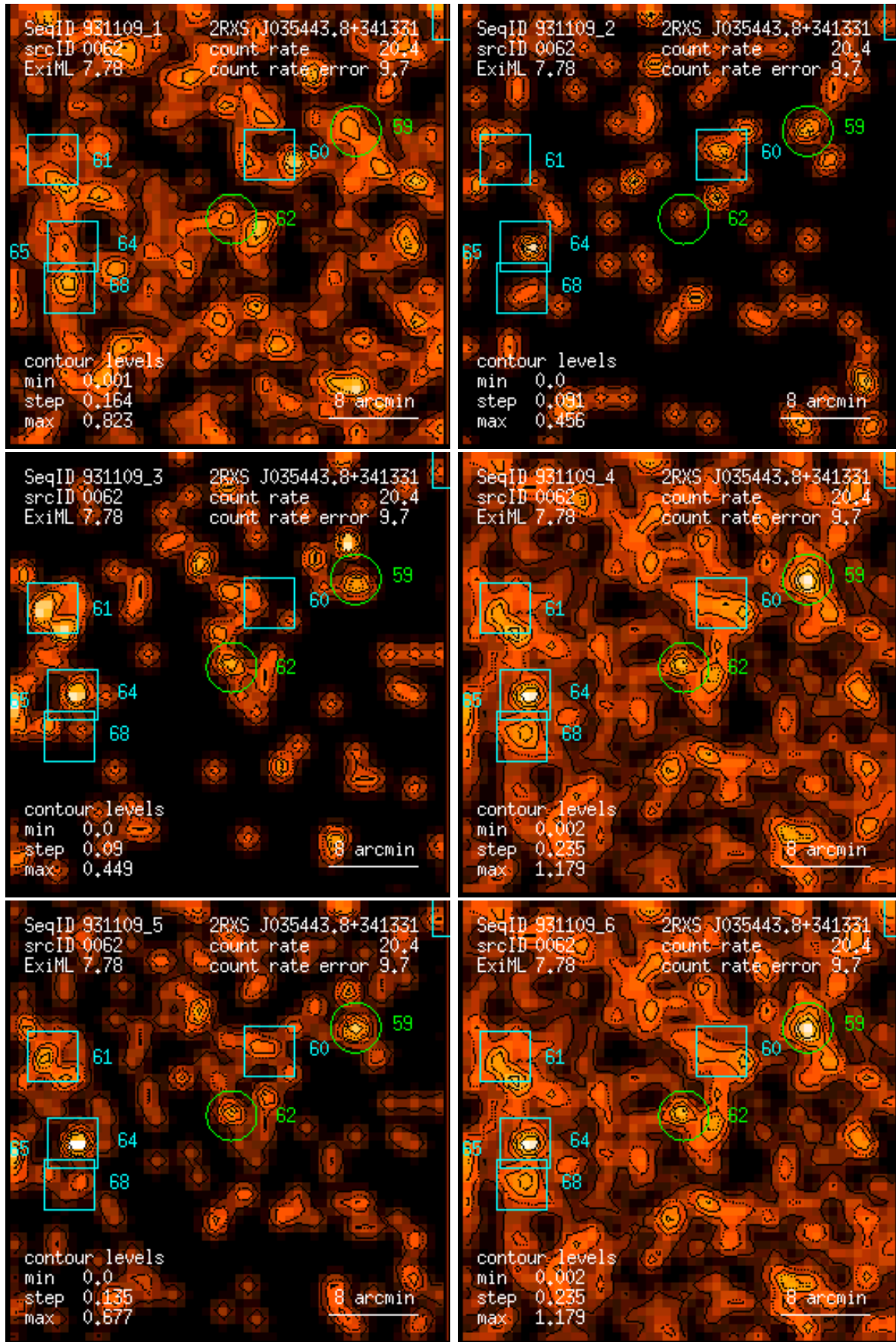
Figure 62: RASS 931109: detection 0062: band rate images, Gaussian filter: (1) PSPC channels 11 – 41, (2) 52 – 90, (3) 91 – 201, (4) 11 – 235, (5) 52 – 201, (6) 11 – 201. Broad band rates in counts/ks. Band rate contour levels in counts/ks/arcmin 2 .
