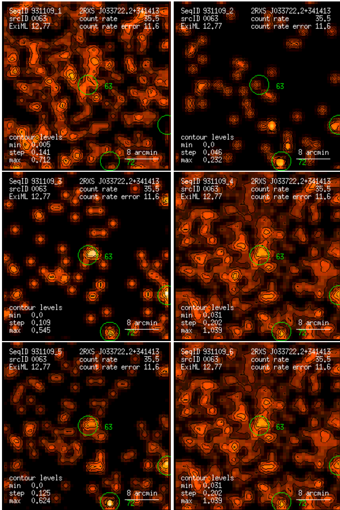
Figure 63: RASS 931109: detection 0063: band rate images, Gaussian filter: (1) PSPC channels 11 – 41, (2) 52 – 90, (3) 91 – 201, (4) 11 – 235, (5) 52 – 201, (6) 11 – 201. Broad band rates in counts/ks. Band rate contour levels in counts/ks/arcmin 2 .
