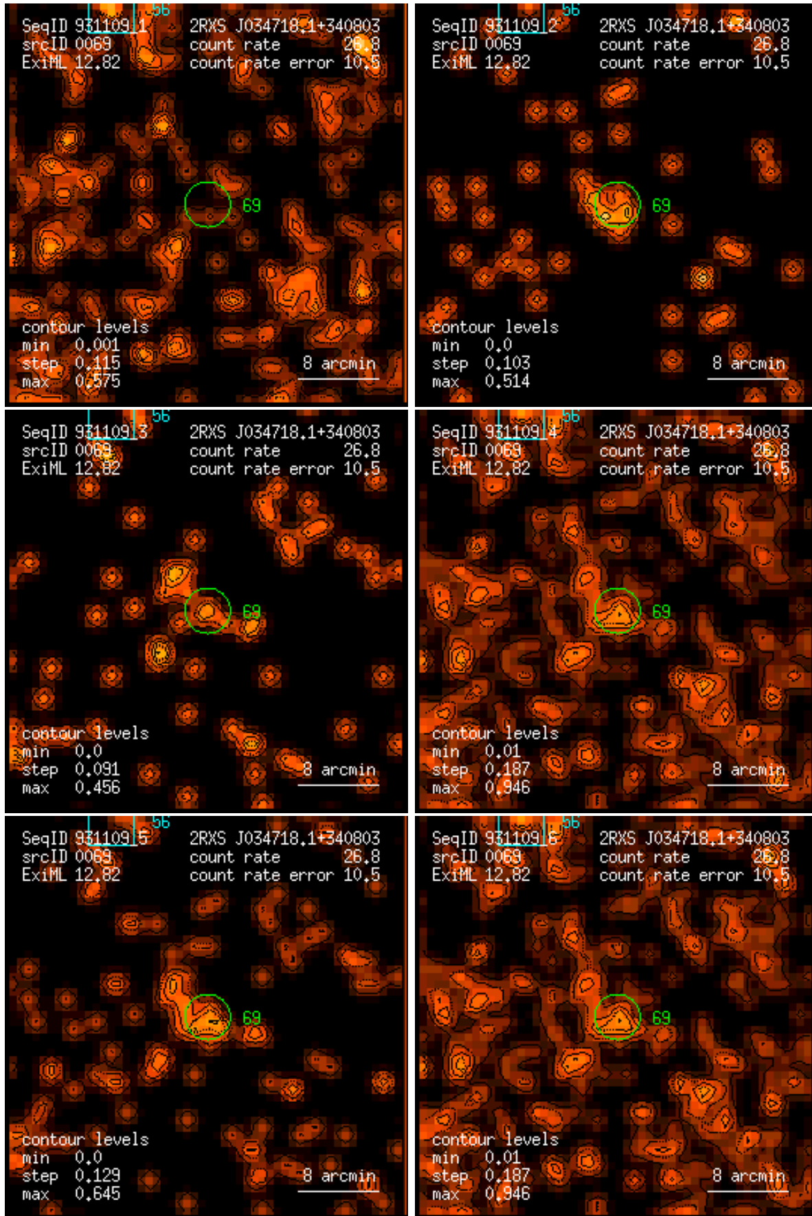
Figure 69: RASS 931109: detection 0069: band rate images, Gaussian filter: (1) PSPC channels 11 – 41, (2) 52 – 90, (3) 91 – 201, (4) 11 – 235, (5) 52 – 201, (6) 11 – 201. Broad band rates in counts/ks. Band rate contour levels in counts/ks/arcmin 2 .
