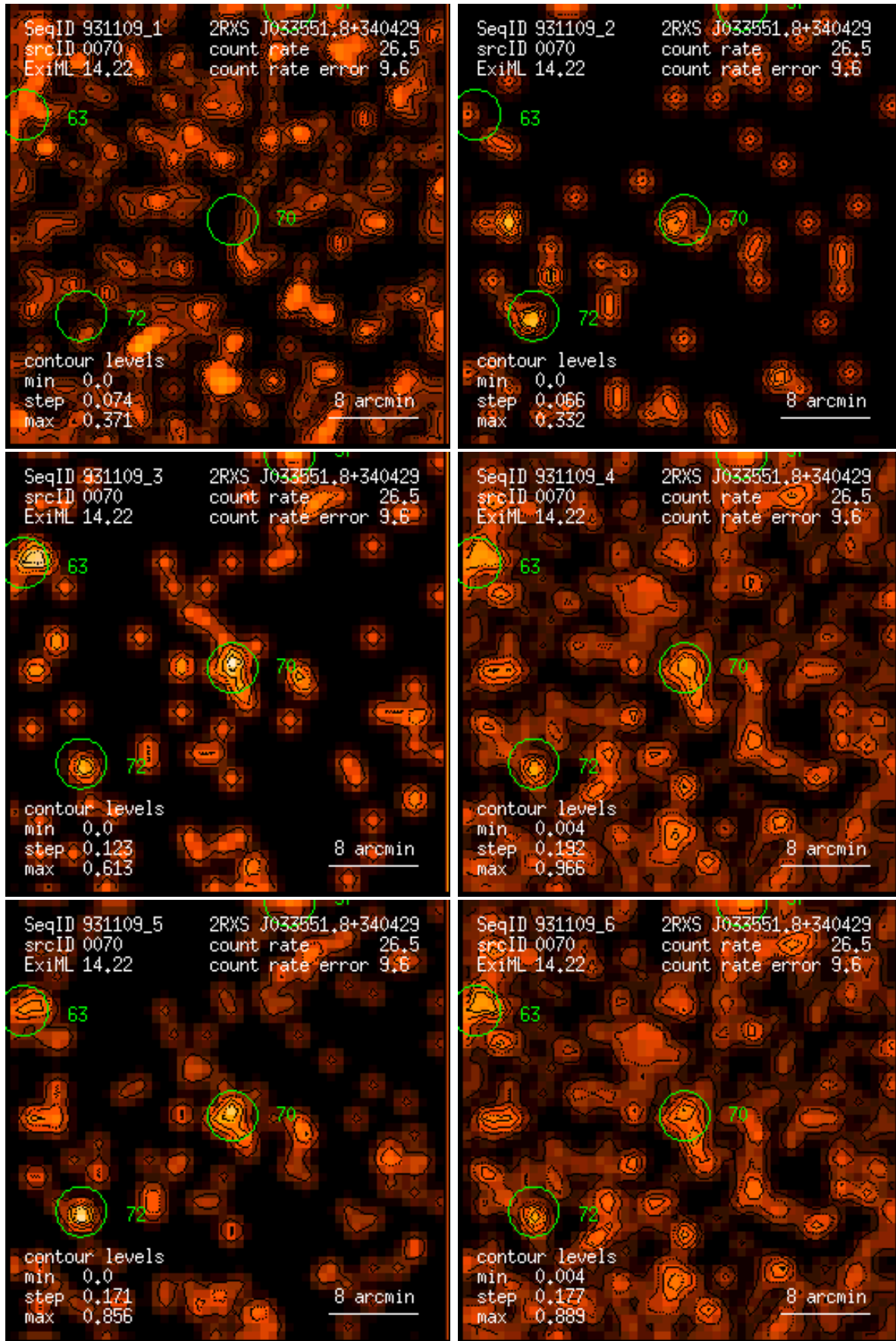
Figure 70: RASS 931109: detection 0070: band rate images, Gaussian filter: (1) PSPC channels 11 – 41, (2) 52 – 90, (3) 91 – 201, (4) 11 – 235, (5) 52 – 201, (6) 11 – 201. Broad band rates in counts/ks. Band rate contour levels in counts/ks/arcmin 2 .
