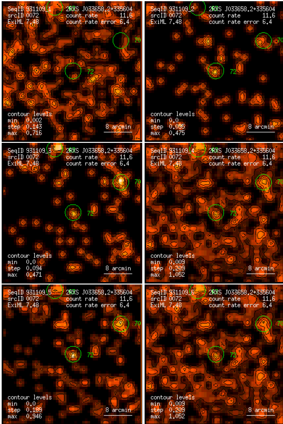
Figure 72: RASS 931109: detection 0072: band rate images, Gaussian filter: (1) PSPC channels 11 – 41, (2) 52 – 90, (3) 91 – 201, (4) 11 – 235, (5) 52 – 201, (6) 11 – 201. Broad band rates in counts/ks. Band rate contour levels in counts/ks/arcmin 2 .
