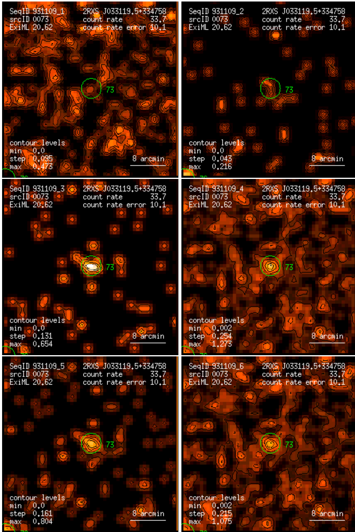
Figure 73: RASS 931109: detection 0073: band rate images, Gaussian filter: (1) PSPC channels 11 – 41, (2) 52 – 90, (3) 91 – 201, (4) 11 – 235, (5) 52 – 201, (6) 11 – 201. Broad band rates in counts/ks. Band rate contour levels in counts/ks/arcmin 2 .
