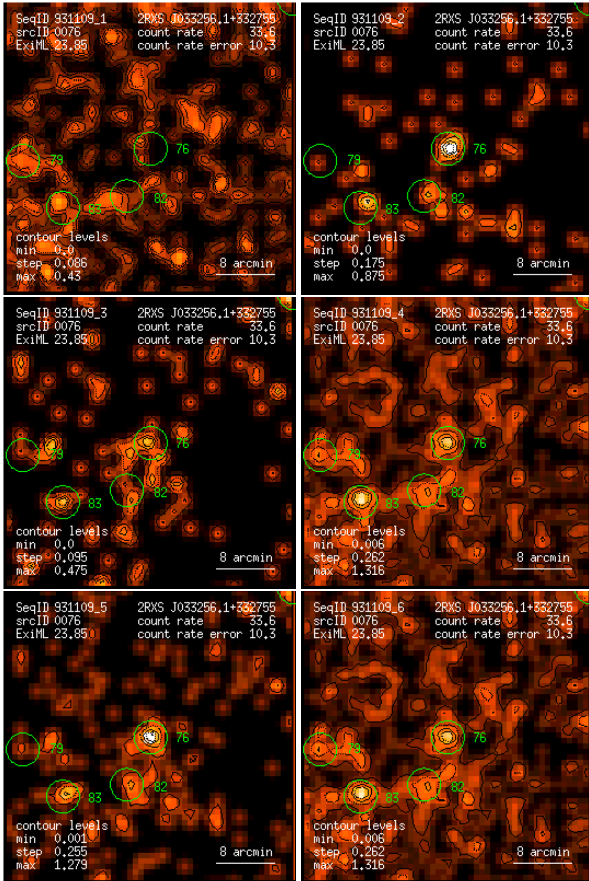
Figure 76: RASS 931109: detection 0076: band rate images, Gaussian filter: (1) PSPC channels 11 – 41, (2) 52 – 90, (3) 91 – 201, (4) 11 – 235, (5) 52 – 201, (6) 11 – 201. Broad band rates in counts/ks. Band rate contour levels in counts/ks/arcmin 2 .
