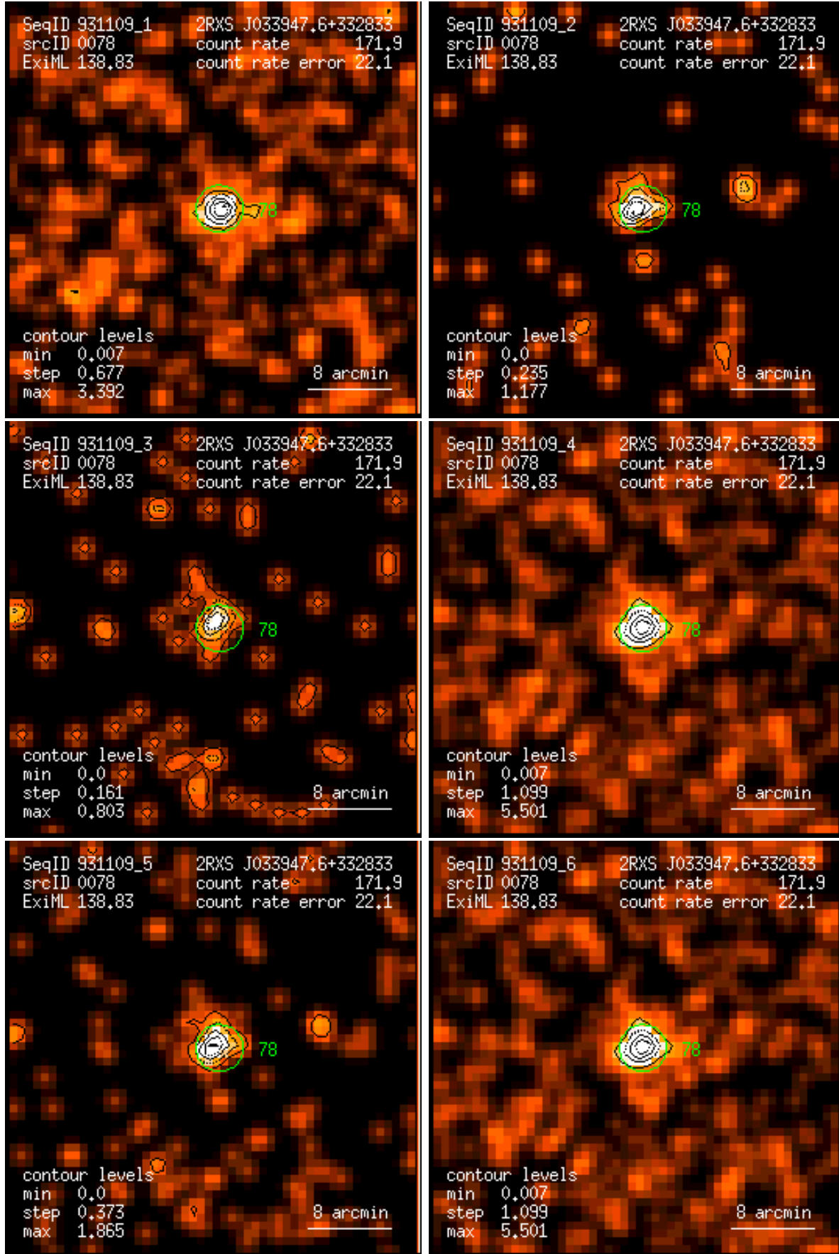
Figure 78: RASS 931109: detection 0078: band rate images, Gaussian filter: (1) PSPC channels 11 – 41, (2) 52 – 90, (3) 91 – 201, (4) 11 – 235, (5) 52 – 201, (6) 11 – 201. Broad band rates in counts/ks. Band rate contour levels in counts/ks/arcmin 2 .
