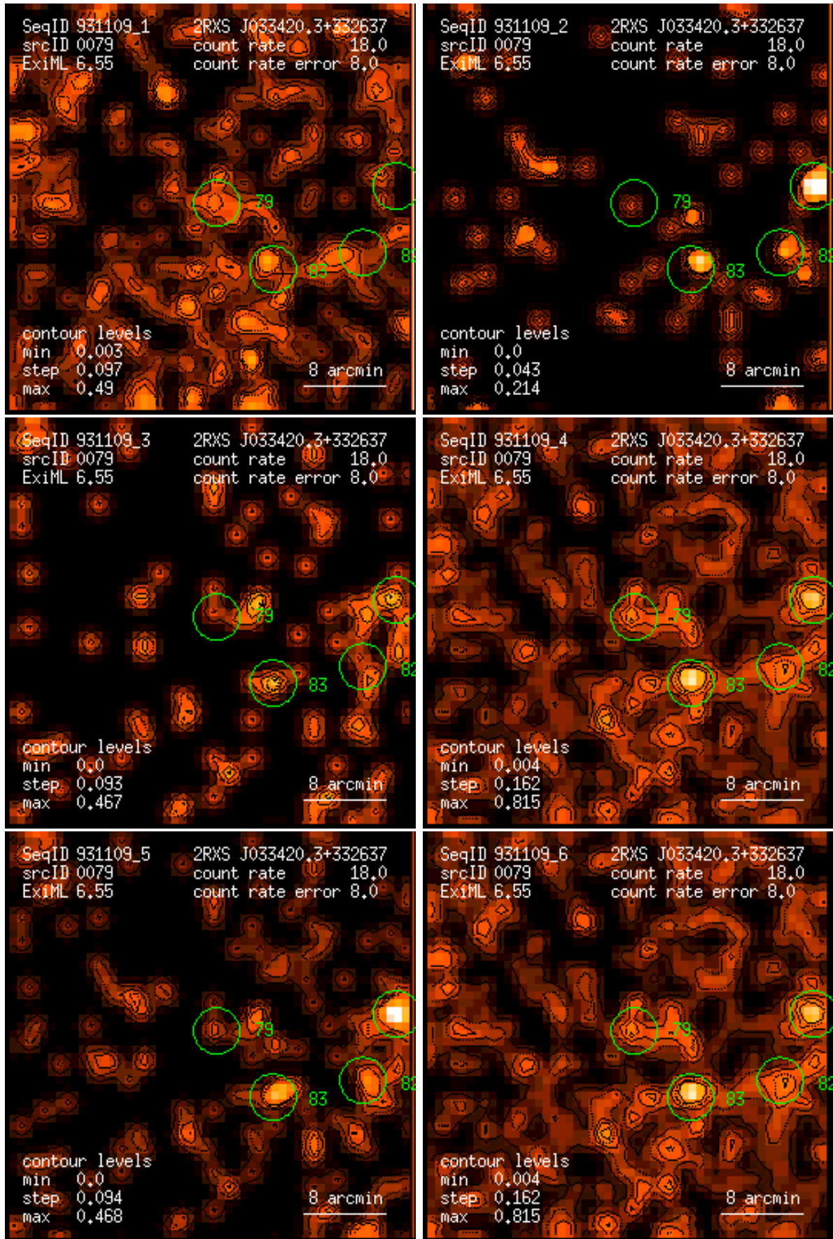
Figure 79: RASS 931109: detection 0079: band rate images, Gaussian filter: (1) PSPC channels 11 – 41, (2) 52 – 90, (3) 91 – 201, (4) 11 – 235, (5) 52 – 201, (6) 11 – 201. Broad band rates in counts/ks. Band rate contour levels in counts/ks/arcmin 2 .
