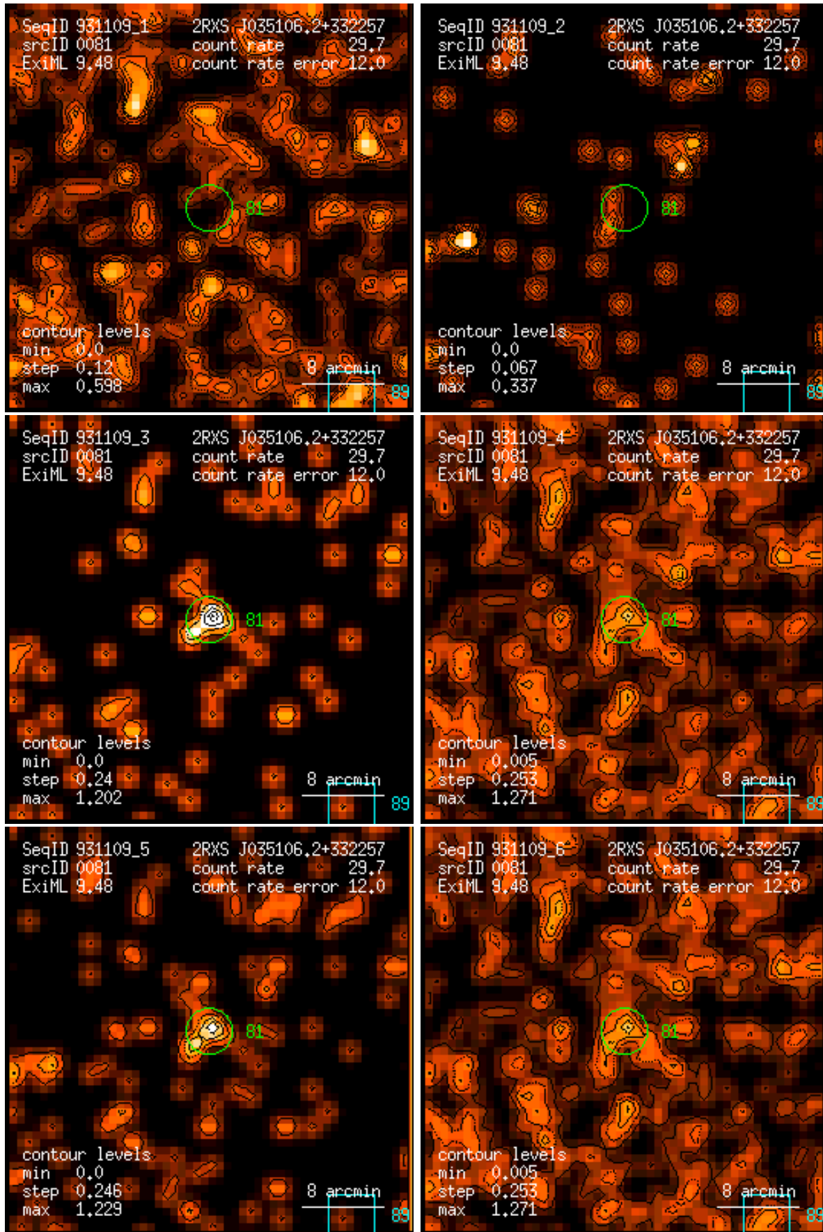
Figure 81: RASS 931109: detection 0081: band rate images, Gaussian filter: (1) PSPC channels 11 – 41, (2) 52 – 90, (3) 91 – 201, (4) 11 – 235, (5) 52 – 201, (6) 11 – 201. Broad band rates in counts/ks. Band rate contour levels in counts/ks/arcmin 2 .
