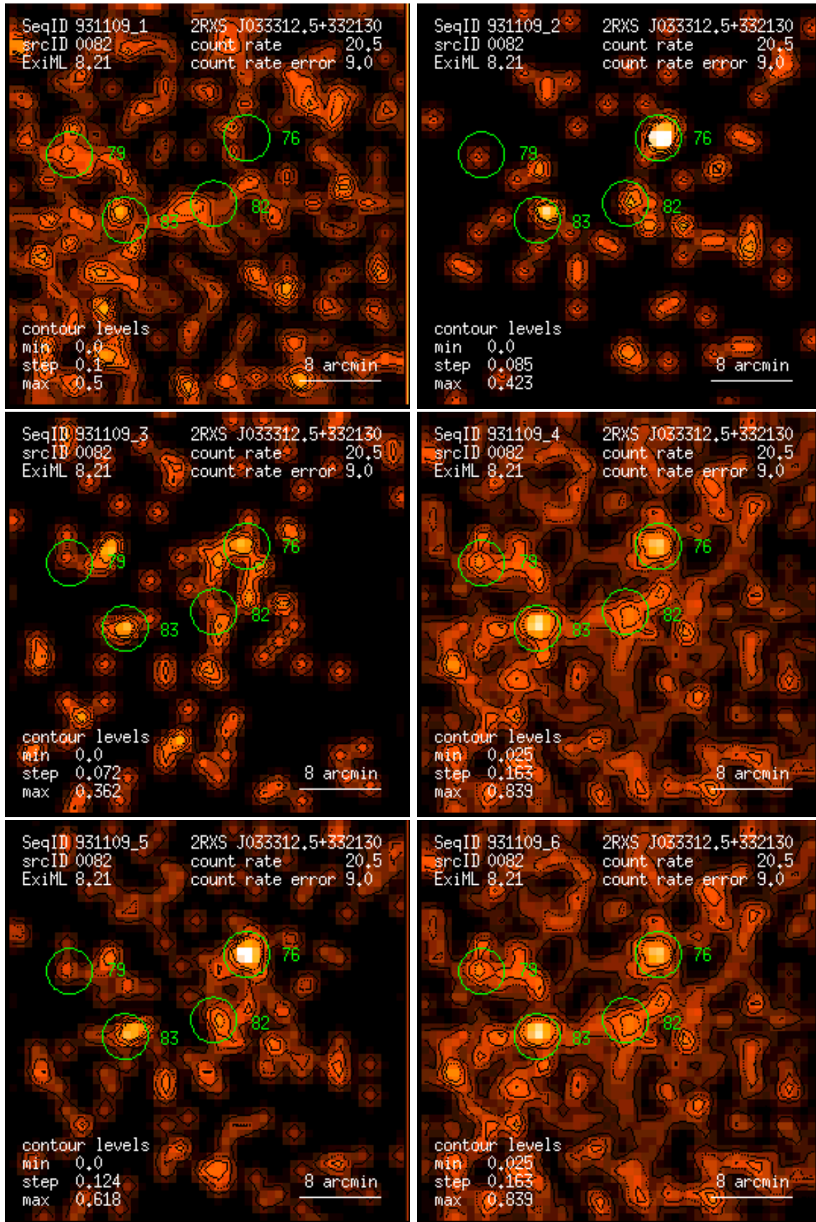
Figure 82: RASS 931109: detection 0082: band rate images, Gaussian filter: (1) PSPC channels 11 – 41, (2) 52 – 90, (3) 91 – 201, (4) 11 – 235, (5) 52 – 201, (6) 11 – 201. Broad band rates in counts/ks. Band rate contour levels in counts/ks/arcmin 2 .
