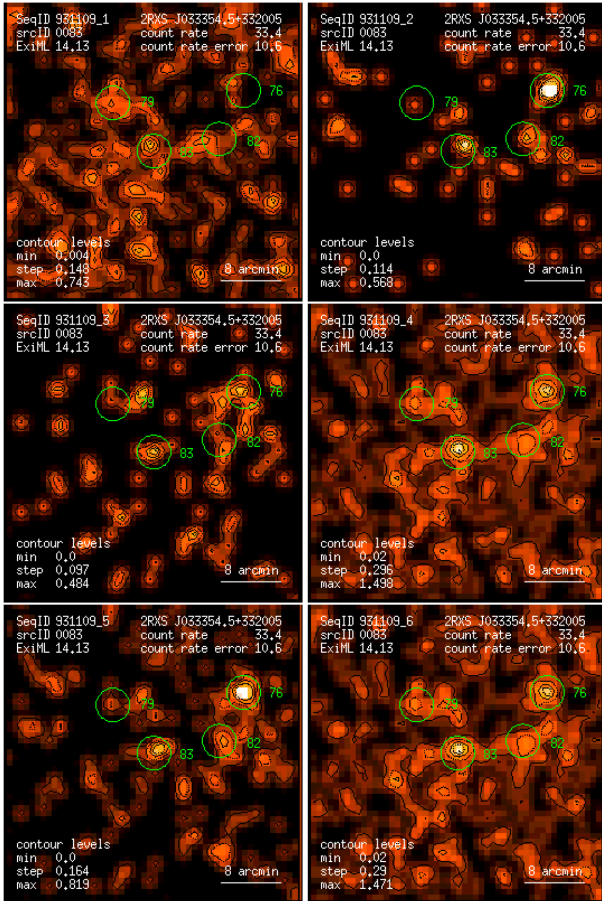
Figure 83: RASS 931109: detection 0083: band rate images, Gaussian filter: (1) PSPC channels 11 – 41, (2) 52 – 90, (3) 91 – 201, (4) 11 – 235, (5) 52 – 201, (6) 11 – 201. Broad band rates in counts/ks. Band rate contour levels in counts/ks/arcmin 2 .
