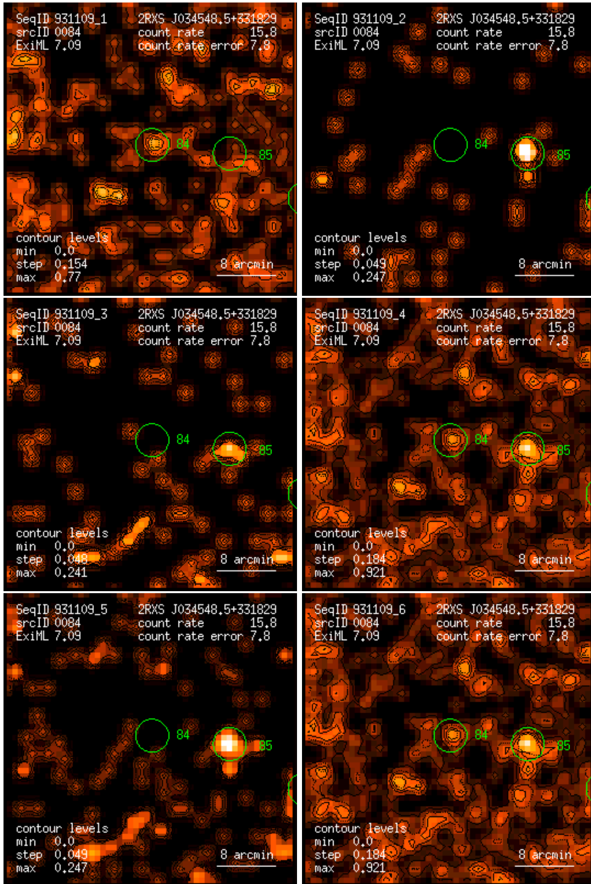
Figure 84: RASS 931109: detection 0084: band rate images, Gaussian filter: (1) PSPC channels 11 – 41, (2) 52 – 90, (3) 91 – 201, (4) 11 – 235, (5) 52 – 201, (6) 11 – 201. Broad band rates in counts/ks. Band rate contour levels in counts/ks/arcmin 2 .
