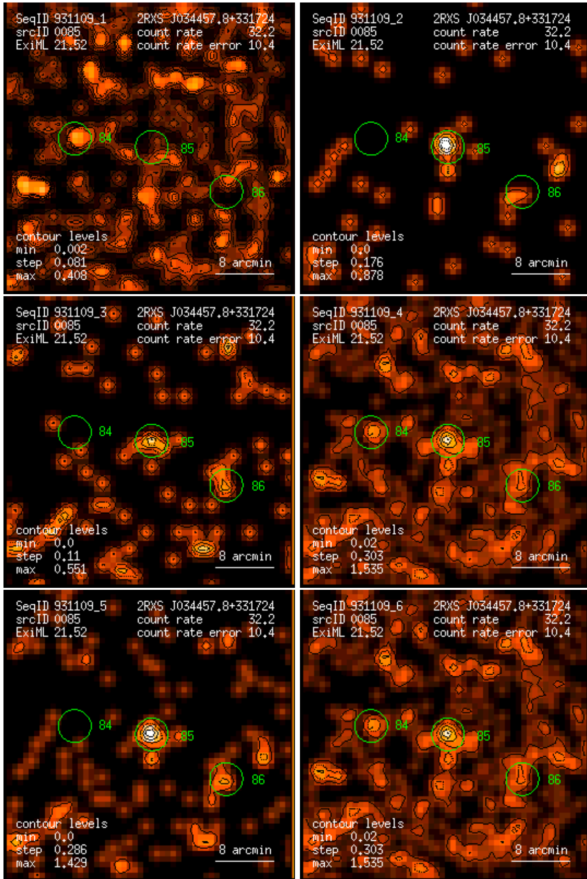
Figure 85: RASS 931109: detection 0085: band rate images, Gaussian filter: (1) PSPC channels 11 – 41, (2) 52 – 90, (3) 91 – 201, (4) 11 – 235, (5) 52 – 201, (6) 11 – 201. Broad band rates in counts/ks. Band rate contour levels in counts/ks/arcmin 2 .
