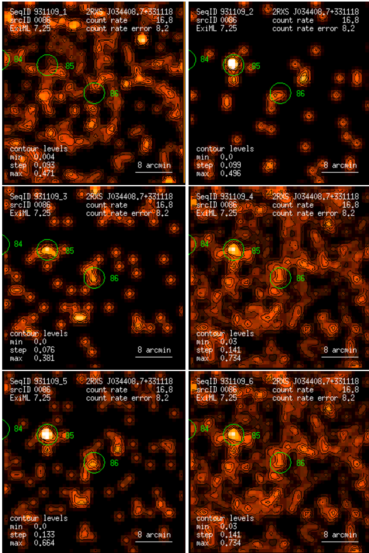
Figure 86: RASS 931109: detection 0086: band rate images, Gaussian filter: (1) PSPC channels 11 – 41, (2) 52 – 90, (3) 91 – 201, (4) 11 – 235, (5) 52 – 201, (6) 11 – 201. Broad band rates in counts/ks. Band rate contour levels in counts/ks/arcmin 2 .
