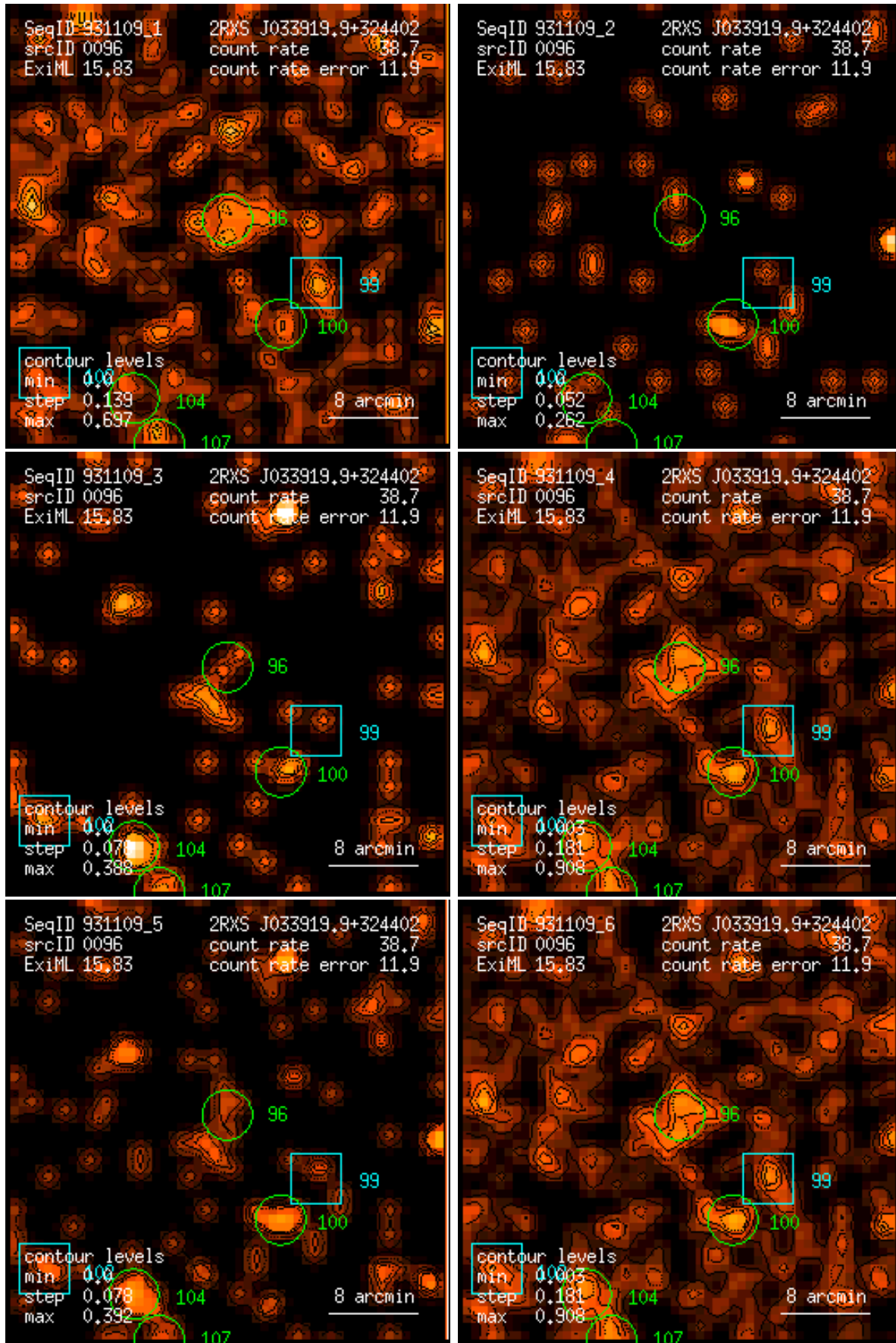
Figure 96: RASS 931109: detection 0096: band rate images, Gaussian filter: (1) PSPC channels 11 – 41, (2) 52 – 90, (3) 91 – 201, (4) 11 – 235, (5) 52 – 201, (6) 11 – 201. Broad band rates in counts/ks. Band rate contour levels in counts/ks/arcmin 2 .
