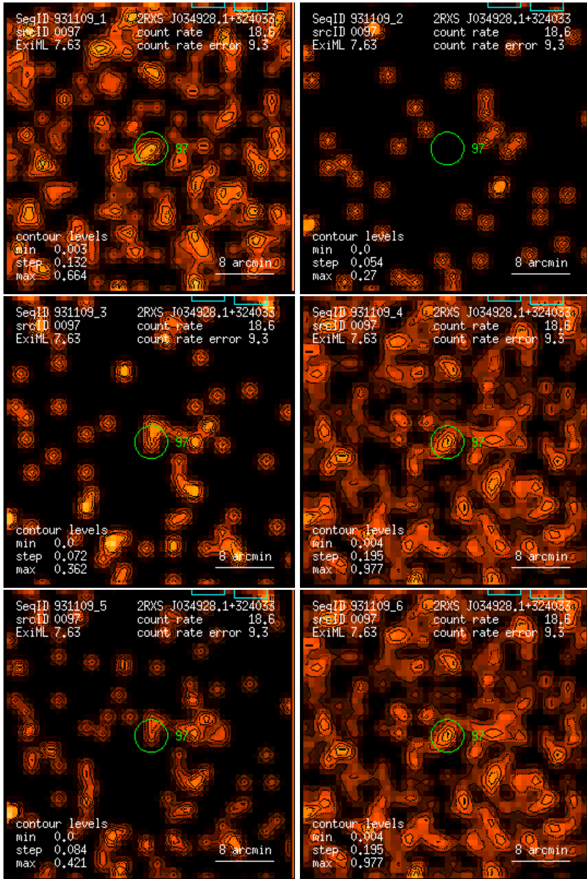
Figure 97: RASS 931109: detection 0097: band rate images, Gaussian filter: (1) PSPC channels 11 – 41, (2) 52 – 90, (3) 91 – 201, (4) 11 – 235, (5) 52 – 201, (6) 11 – 201. Broad band rates in counts/ks. Band rate contour levels in counts/ks/arcmin 2 .
