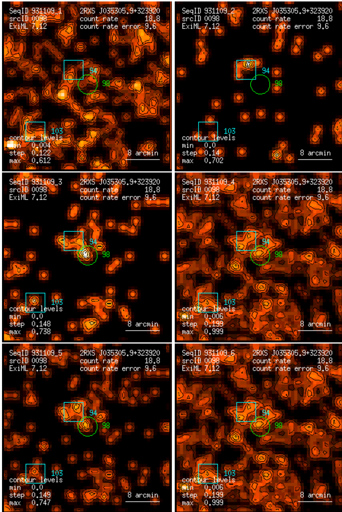
Figure 98: RASS 931109: detection 0098: band rate images, Gaussian filter: (1) PSPC channels 11 – 41, (2) 52 – 90, (3) 91 – 201, (4) 11 – 235, (5) 52 – 201, (6) 11 – 201. Broad band rates in counts/ks. Band rate contour levels in counts/ks/arcmin 2 .
