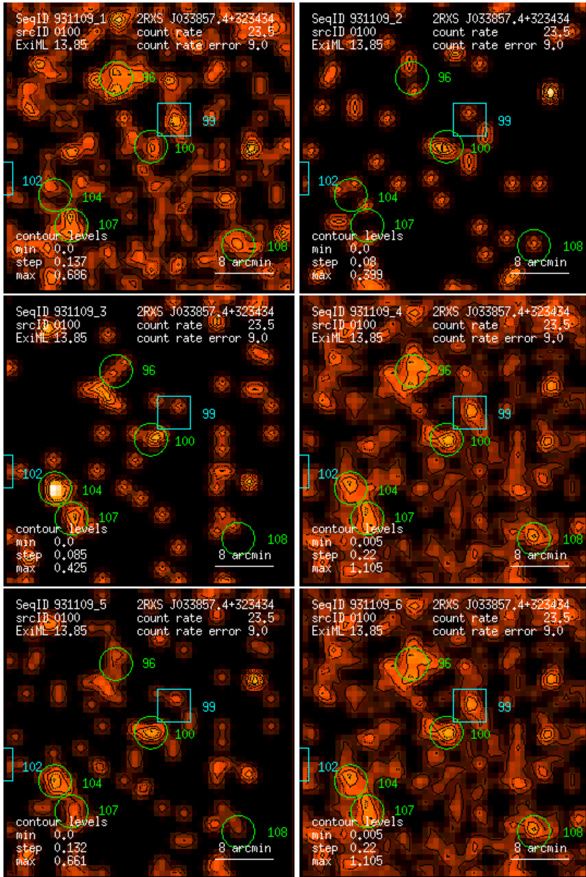
Figure 100: RASS 931109: detection 0100: band rate images, Gaussian filter: (1) PSPC channels 11 – 41, (2) 52 – 90, (3) 91 – 201, (4) 11 – 235, (5) 52 – 201, (6) 11 – 201. Broad band rates in counts/ks. Band rate contour levels in counts/ks/arcmin 2 .
