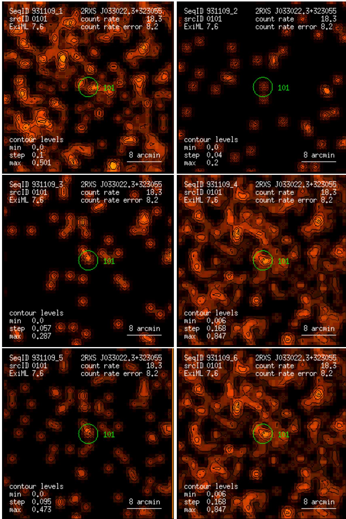
Figure 101: RASS 931109: detection 0101: band rate images, Gaussian filter: (1) PSPC channels 11 – 41, (2) 52 – 90, (3) 91 – 201, (4) 11 – 235, (5) 52 – 201, (6) 11 – 201. Broad band rates in counts/ks. Band rate contour levels in counts/ks/arcmin 2 .
