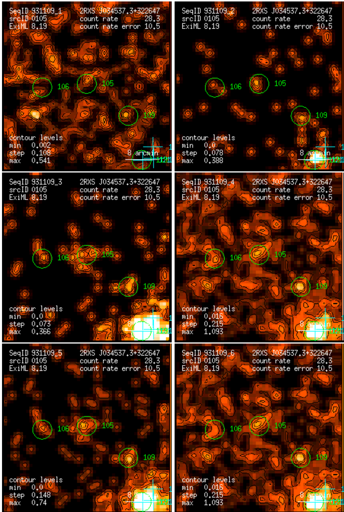
Figure 105: RASS 931109: detection 0105: band rate images, Gaussian filter: (1) PSPC channels 11 – 41, (2) 52 – 90, (3) 91 – 201, (4) 11 – 235, (5) 52 – 201, (6) 11 – 201. Broad band rates in counts/ks. Band rate contour levels in counts/ks/arcmin 2 .
