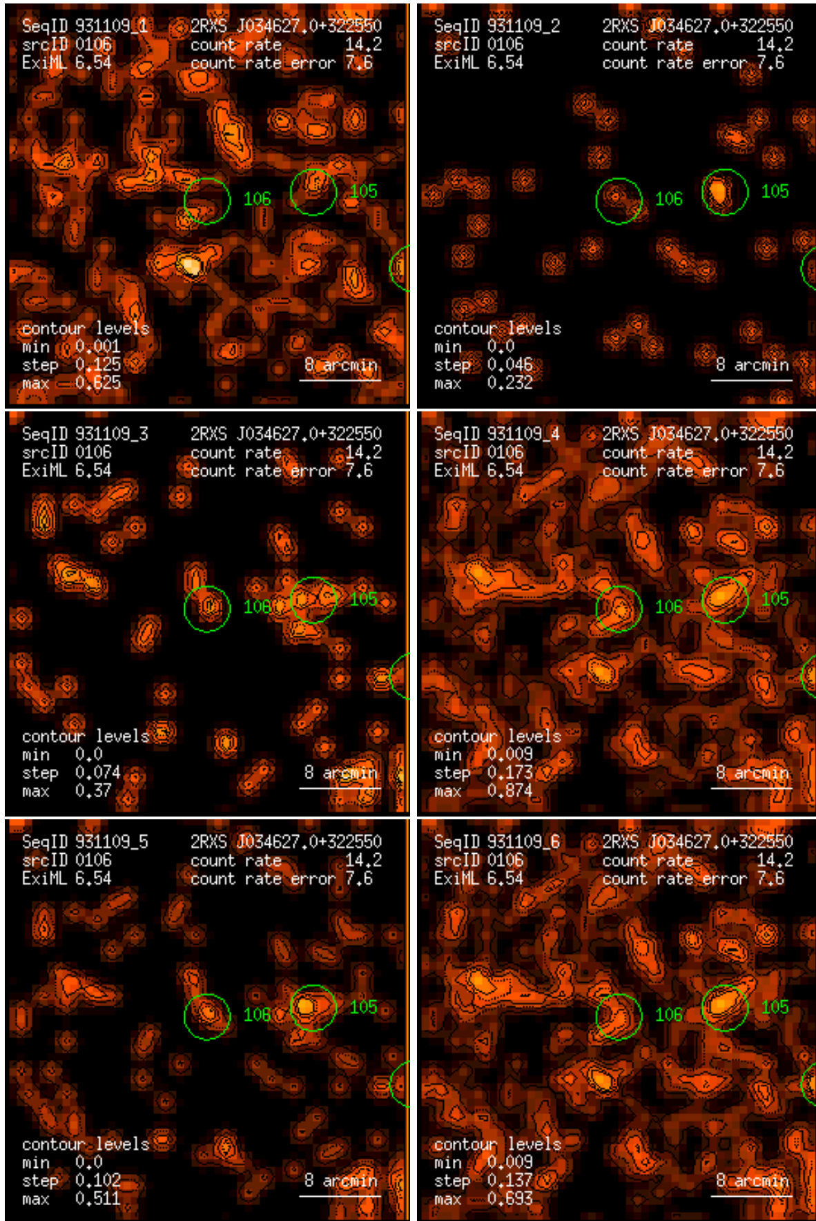
Figure 106: RASS 931109: detection 0106: band rate images, Gaussian filter: (1) PSPC channels 11 – 41, (2) 52 – 90, (3) 91 – 201, (4) 11 – 235, (5) 52 – 201, (6) 11 – 201. Broad band rates in counts/ks. Band rate contour levels in counts/ks/arcmin 2 .
