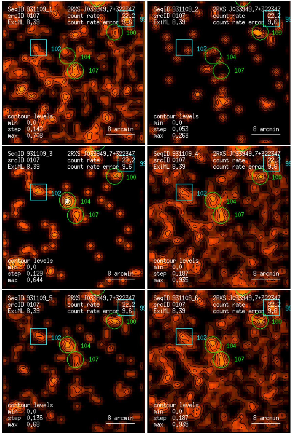
Figure 107: RASS 931109: detection 0107: band rate images, Gaussian filter: (1) PSPC channels 11 – 41, (2) 52 – 90, (3) 91 – 201, (4) 11 – 235, (5) 52 – 201, (6) 11 – 201. Broad band rates in counts/ks. Band rate contour levels in counts/ks/arcmin 2 .
