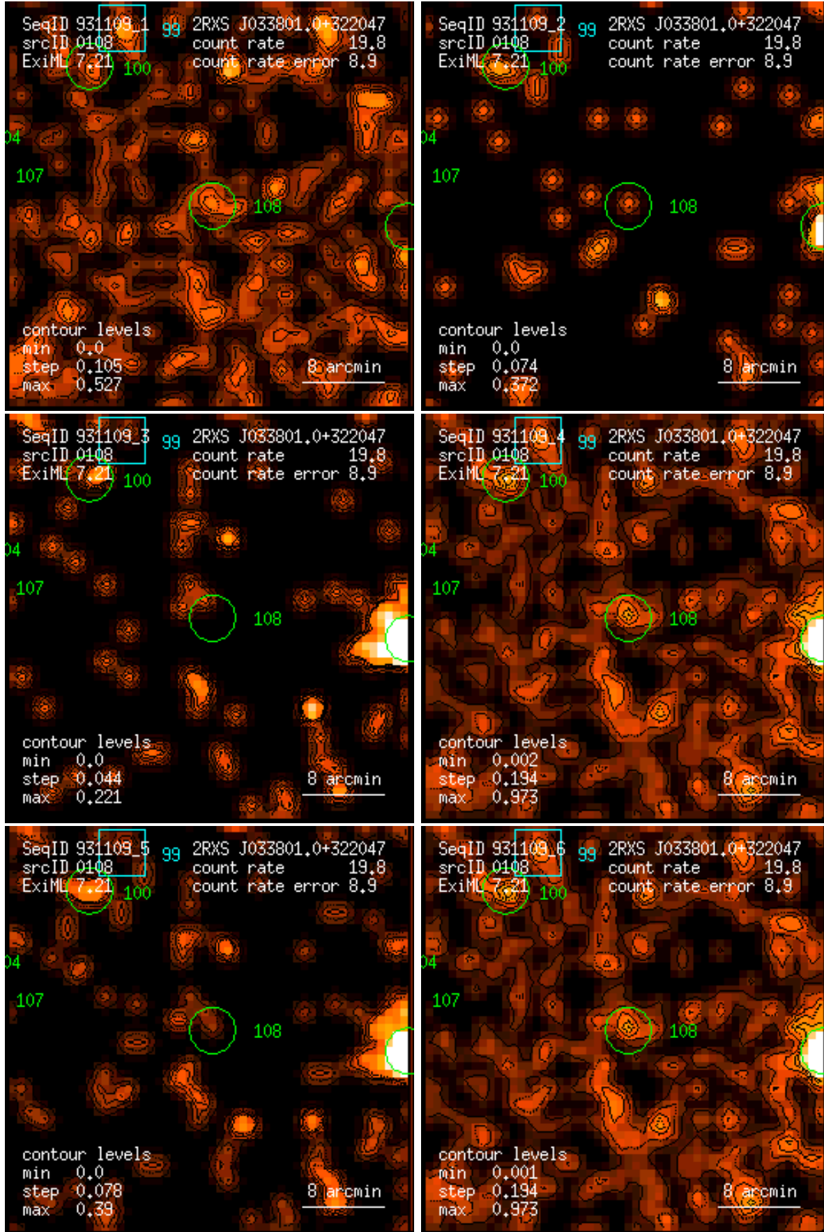
Figure 108: RASS 931109: detection 0108: band rate images, Gaussian filter: (1) PSPC channels 11 – 41, (2) 52 – 90, (3) 91 – 201, (4) 11 – 235, (5) 52 – 201, (6) 11 – 201. Broad band rates in counts/ks. Band rate contour levels in counts/ks/arcmin 2 .
