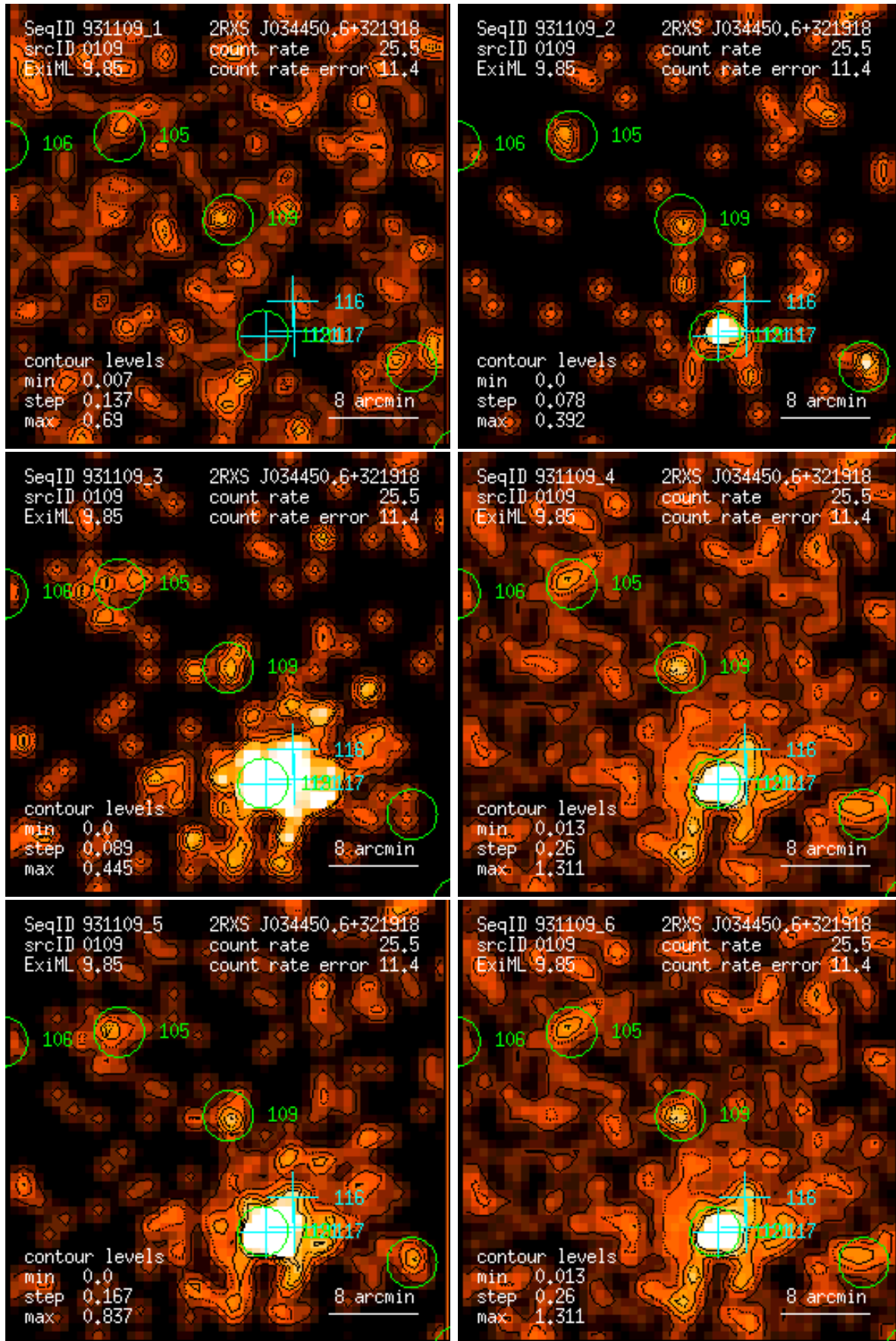
Figure 109: RASS 931109: detection 0109: band rate images, Gaussian filter: (1) PSPC channels 11 – 41, (2) 52 – 90, (3) 91 – 201, (4) 11 – 235, (5) 52 – 201, (6) 11 – 201. Broad band rates in counts/ks. Band rate contour levels in counts/ks/arcmin 2 .
