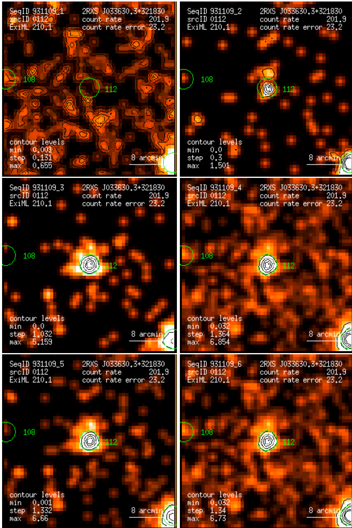
Figure 112: RASS 931109: detection 0112: band rate images, Gaussian filter: (1) PSPC channels 11 – 41, (2) 52 – 90, (3) 91 – 201, (4) 11 – 235, (5) 52 – 201, (6) 11 – 201. Broad band rates in counts/ks. Band rate contour levels in counts/ks/arcmin 2 .
