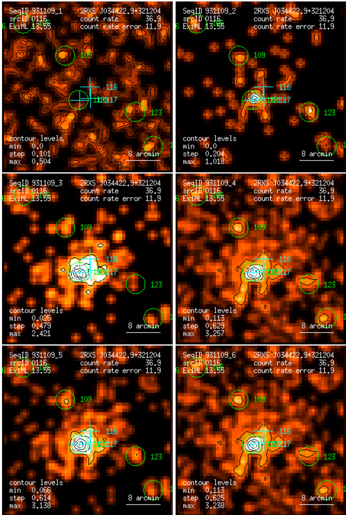
Figure 116: RASS 931109: detection 0116: band rate images, Gaussian filter: (1) PSPC channels 11 – 41, (2) 52 – 90, (3) 91 – 201, (4) 11 – 235, (5) 52 – 201, (6) 11 – 201. Broad band rates in counts/ks. Band rate contour levels in counts/ks/arcmin 2 .
