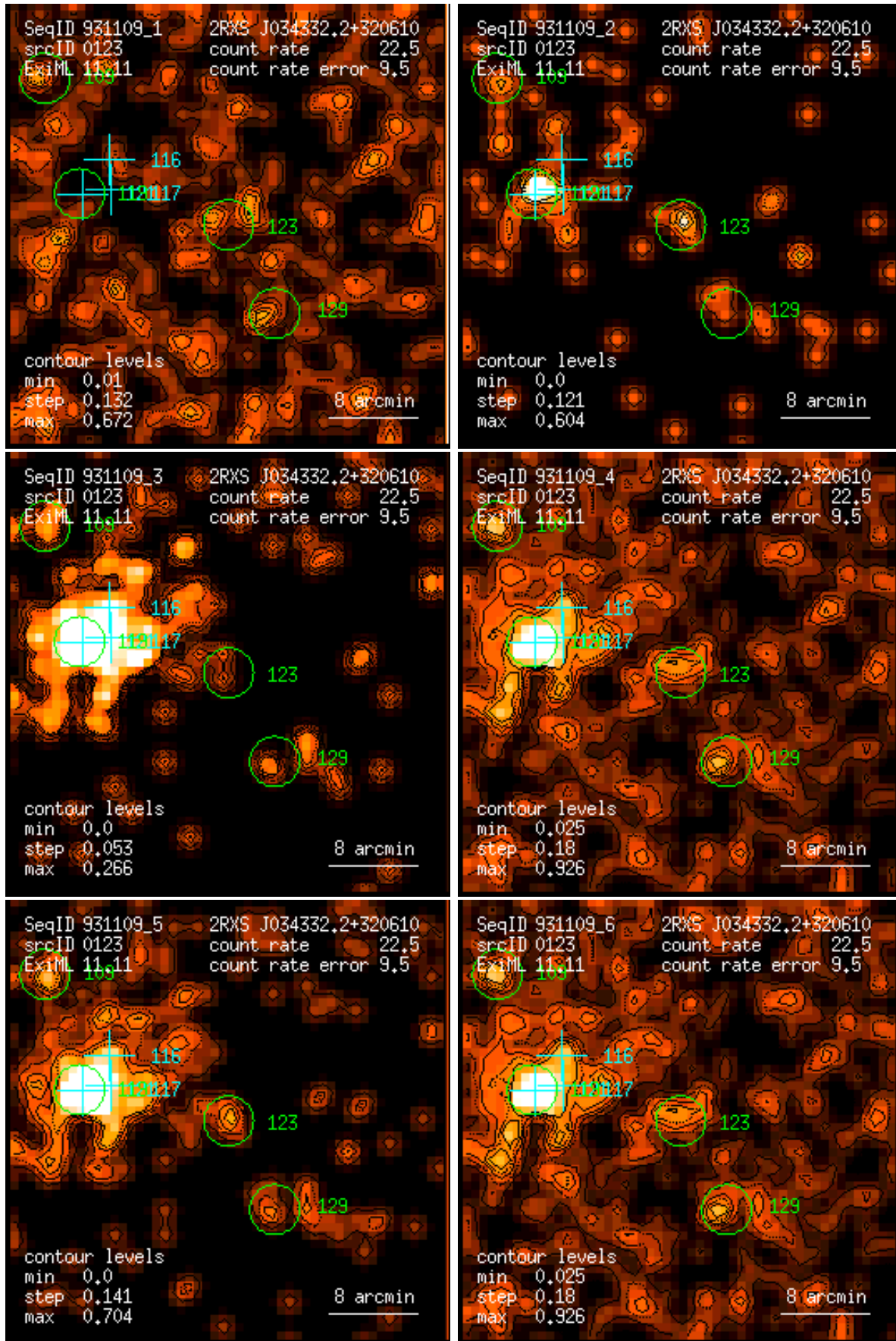
Figure 123: RASS 931109: detection 0123: band rate images, Gaussian filter: (1) PSPC channels 11 – 41, (2) 52 – 90, (3) 91 – 201, (4) 11 – 235, (5) 52 – 201, (6) 11 – 201. Broad band rates in counts/ks. Band rate contour levels in counts/ks/arcmin 2 .
