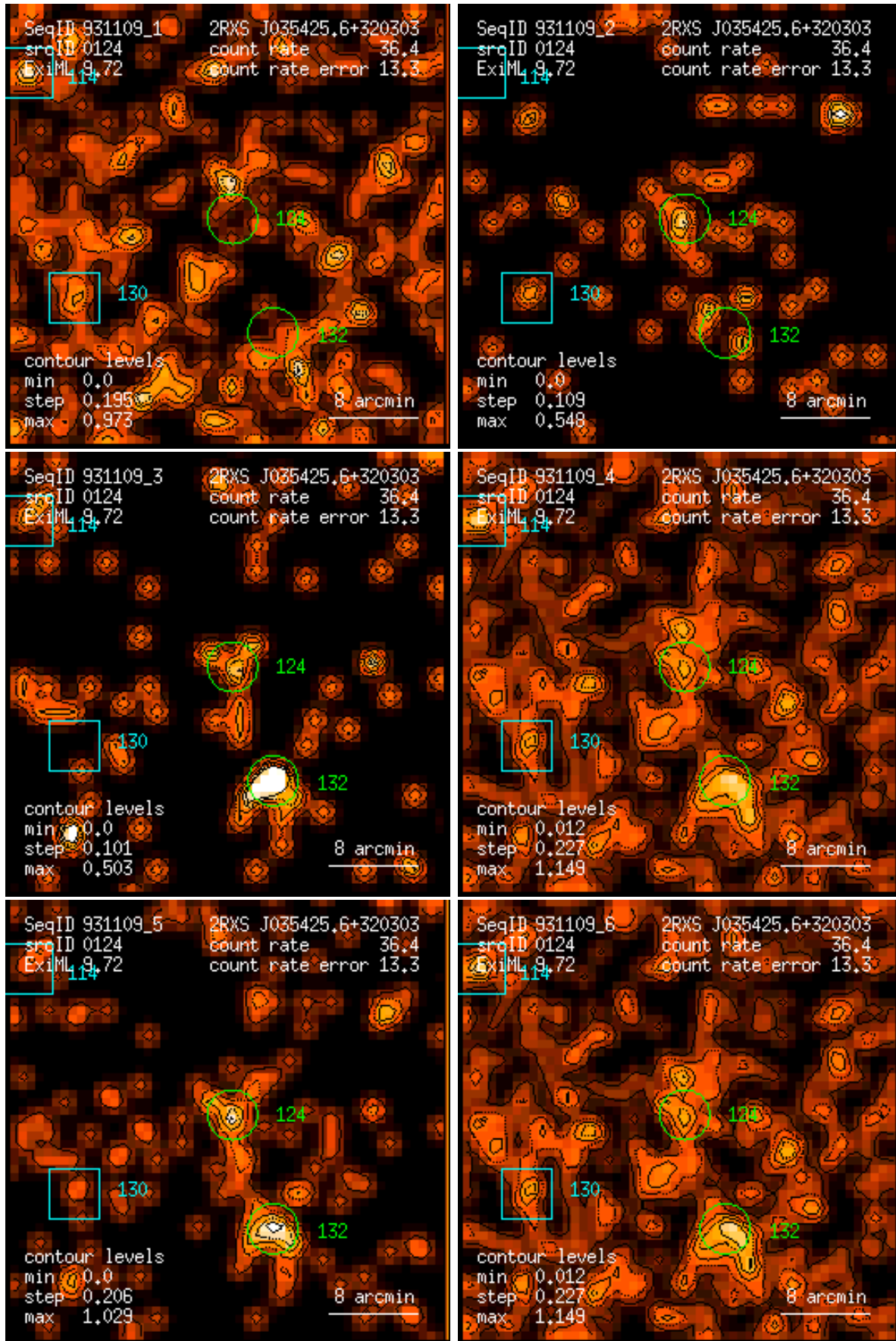
Figure 124: RASS 931109: detection 0124: band rate images, Gaussian filter: (1) PSPC channels 11 – 41, (2) 52 – 90, (3) 91 – 201, (4) 11 – 235, (5) 52 – 201, (6) 11 – 201. Broad band rates in counts/ks. Band rate contour levels in counts/ks/arcmin 2 .
