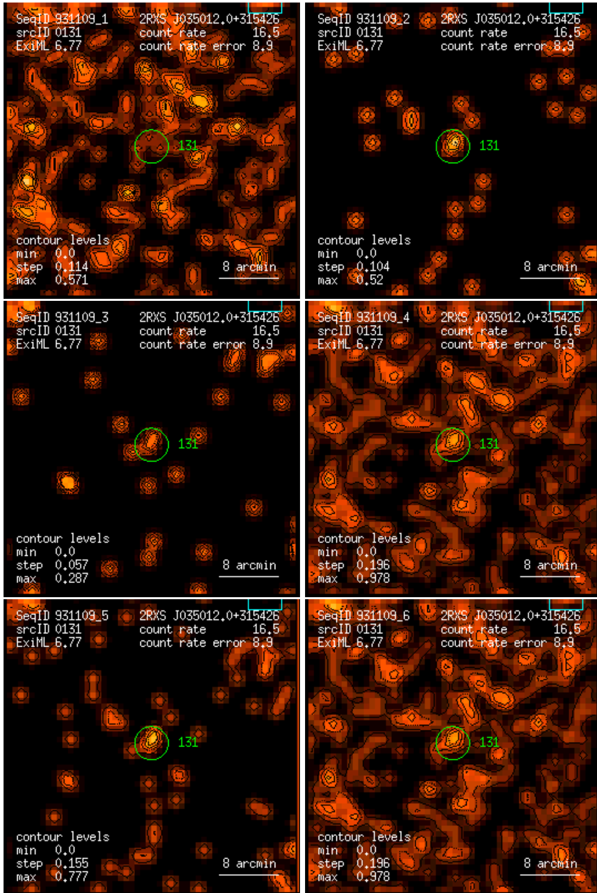
Figure 131: RASS 931109: detection 0131: band rate images, Gaussian filter: (1) PSPC channels 11 – 41, (2) 52 – 90, (3) 91 – 201, (4) 11 – 235, (5) 52 – 201, (6) 11 – 201. Broad band rates in counts/ks. Band rate contour levels in counts/ks/arcmin 2 .
