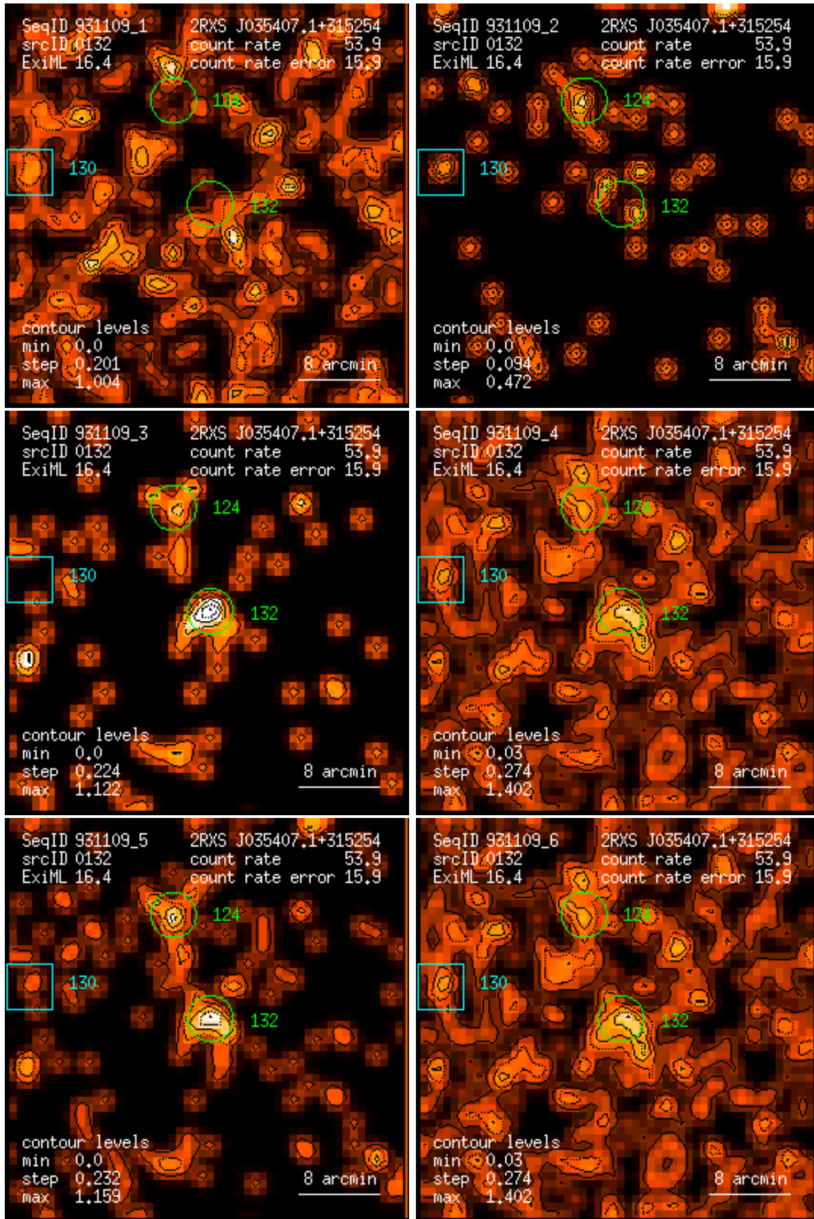
Figure 132: RASS 931109: detection 0132: band rate images, Gaussian filter: (1) PSPC channels 11 – 41, (2) 52 – 90, (3) 91 – 201, (4) 11 – 235, (5) 52 – 201, (6) 11 – 201. Broad band rates in counts/ks. Band rate contour levels in counts/ks/arcmin 2 .
