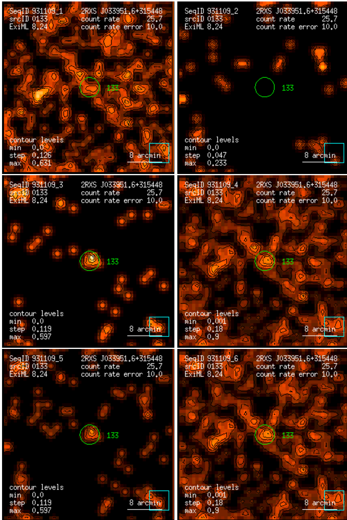
Figure 133: RASS 931109: detection 0133: band rate images, Gaussian filter: (1) PSPC channels 11 – 41, (2) 52 – 90, (3) 91 – 201, (4) 11 – 235, (5) 52 – 201, (6) 11 – 201. Broad band rates in counts/ks. Band rate contour levels in counts/ks/arcmin 2 .
