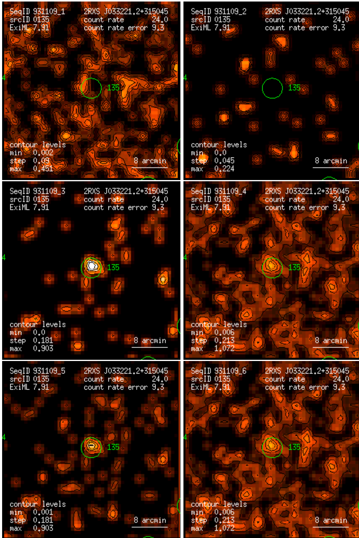
Figure 135: RASS 931109: detection 0135: band rate images, Gaussian filter: (1) PSPC channels 11 – 41, (2) 52 – 90, (3) 91 – 201, (4) 11 – 235, (5) 52 – 201, (6) 11 – 201. Broad band rates in counts/ks. Band rate contour levels in counts/ks/arcmin 2 .
