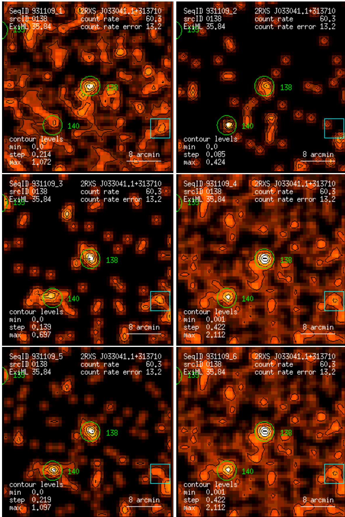
Figure 138: RASS 931109: detection 0138: band rate images, Gaussian filter: (1) PSPC channels 11 – 41, (2) 52 – 90, (3) 91 – 201, (4) 11 – 235, (5) 52 – 201, (6) 11 – 201. Broad band rates in counts/ks. Band rate contour levels in counts/ks/arcmin 2 .
