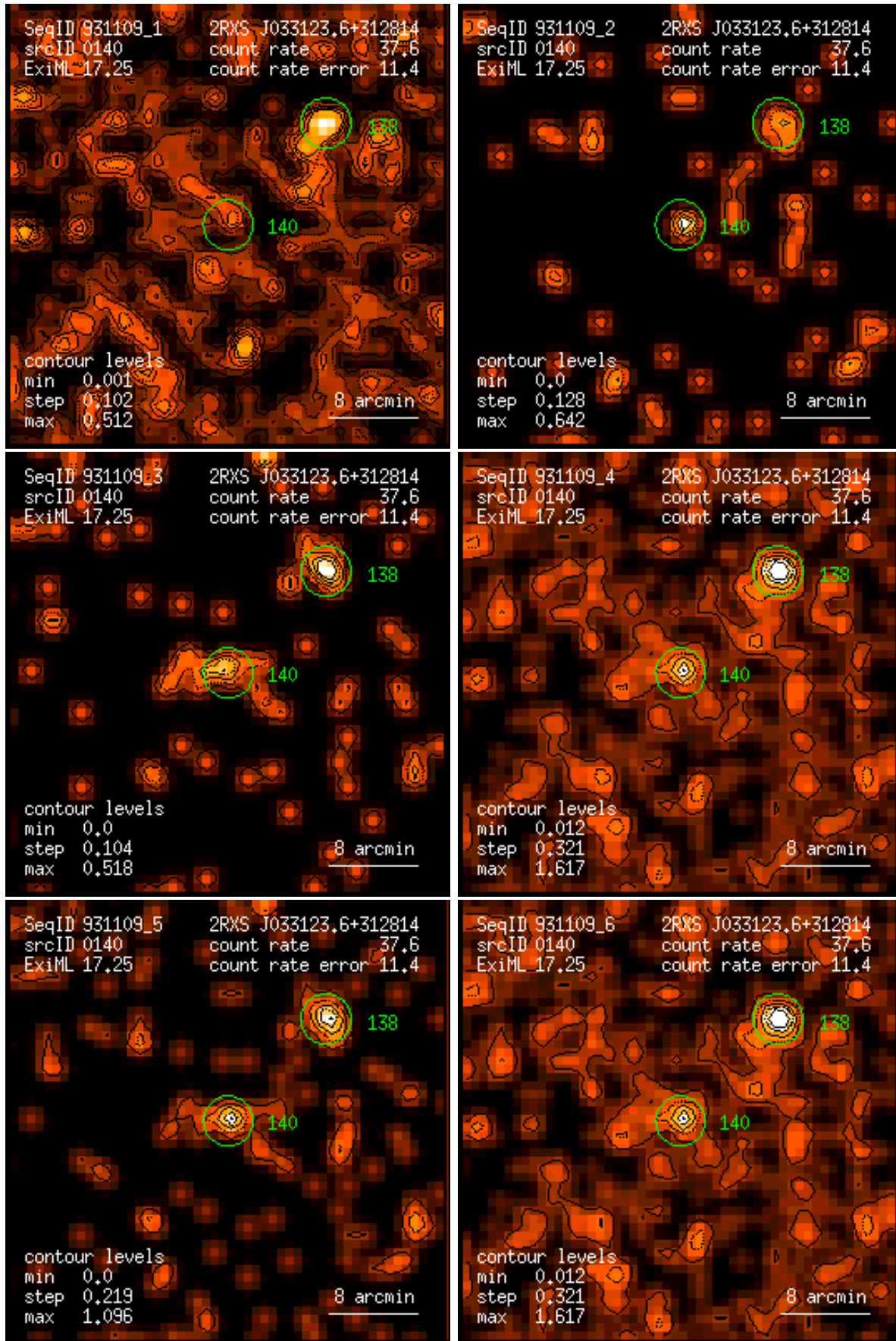
Figure 140: RASS 931109: detection 0140: band rate images, Gaussian filter: (1) PSPC channels 11 – 41, (2) 52 – 90, (3) 91 – 201, (4) 11 – 235, (5) 52 – 201, (6) 11 – 201. Broad band rates in counts/ks. Band rate contour levels in counts/ks/arcmin 2 .
