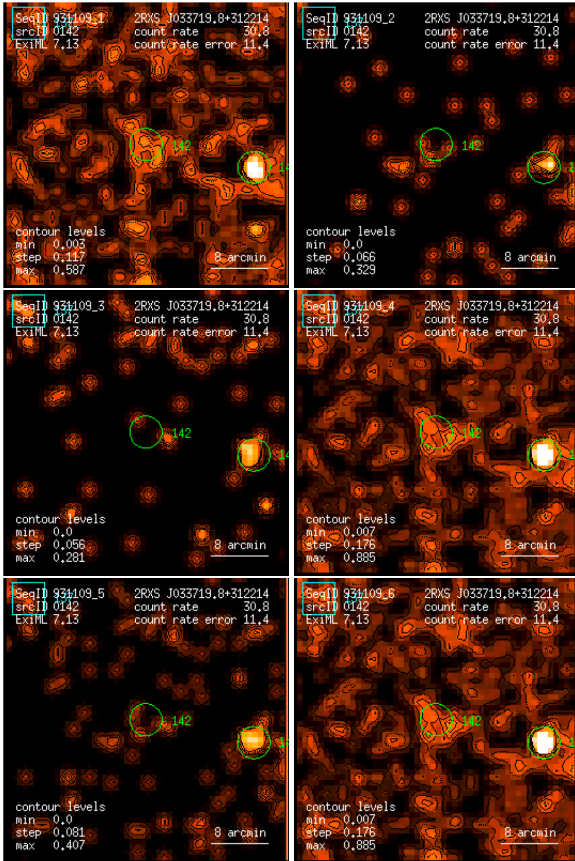
Figure 142: RASS 931109: detection 0142: band rate images, Gaussian filter: (1) PSPC channels 11 – 41, (2) 52 – 90, (3) 91 – 201, (4) 11 – 235, (5) 52 – 201, (6) 11 – 201. Broad band rates in counts/ks. Band rate contour levels in counts/ks/arcmin 2 .
