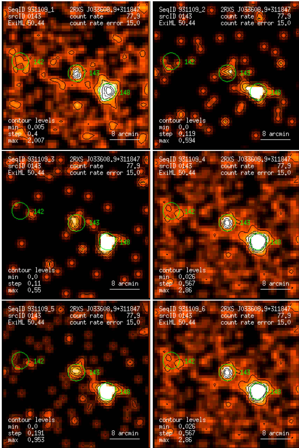
Figure 143: RASS 931109: detection 0143: band rate images, Gaussian filter: (1) PSPC channels 11 – 41, (2) 52 – 90, (3) 91 – 201, (4) 11 – 235, (5) 52 – 201, (6) 11 – 201. Broad band rates in counts/ks. Band rate contour levels in counts/ks/arcmin 2 .
