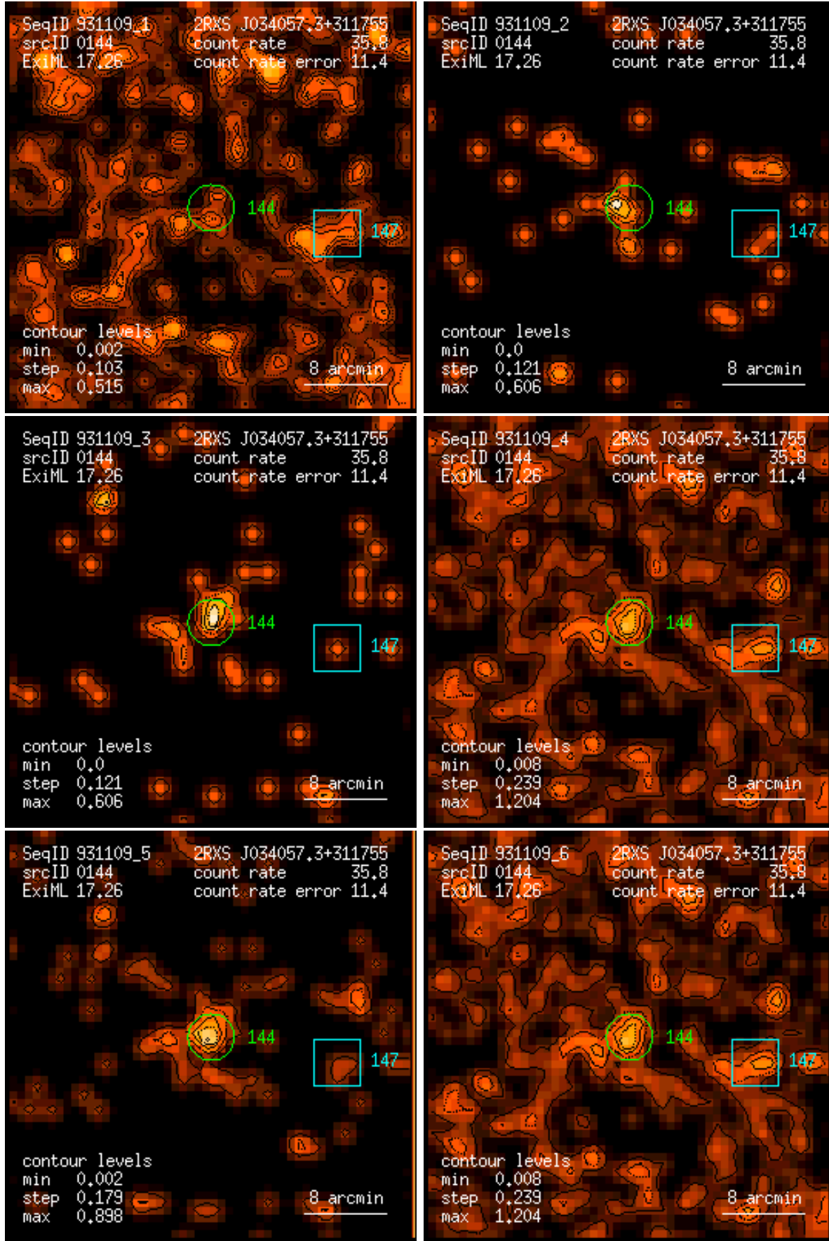
Figure 144: RASS 931109: detection 0144: band rate images, Gaussian filter: (1) PSPC channels 11 – 41, (2) 52 – 90, (3) 91 – 201, (4) 11 – 235, (5) 52 – 201, (6) 11 – 201. Broad band rates in counts/ks. Band rate contour levels in counts/ks/arcmin 2 .
