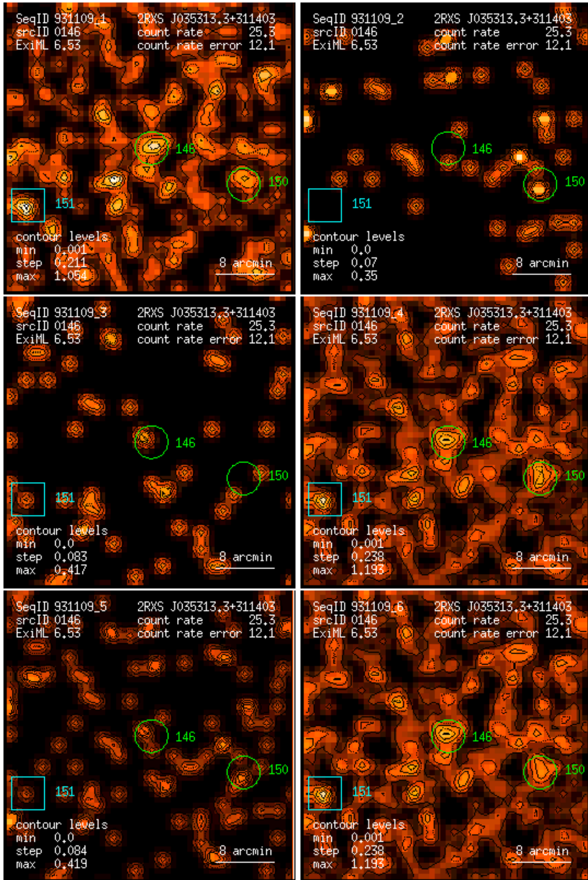
Figure 146: RASS 931109: detection 0146: band rate images, Gaussian filter: (1) PSPC channels 11 – 41, (2) 52 – 90, (3) 91 – 201, (4) 11 – 235, (5) 52 – 201, (6) 11 – 201. Broad band rates in counts/ks. Band rate contour levels in counts/ks/arcmin 2 .
