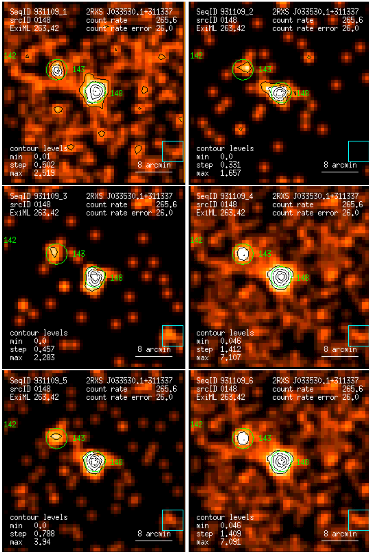
Figure 148: RASS 931109: detection 0148: band rate images, Gaussian filter: (1) PSPC channels 11 – 41, (2) 52 – 90, (3) 91 – 201, (4) 11 – 235, (5) 52 – 201, (6) 11 – 201. Broad band rates in counts/ks. Band rate contour levels in counts/ks/arcmin 2 .
