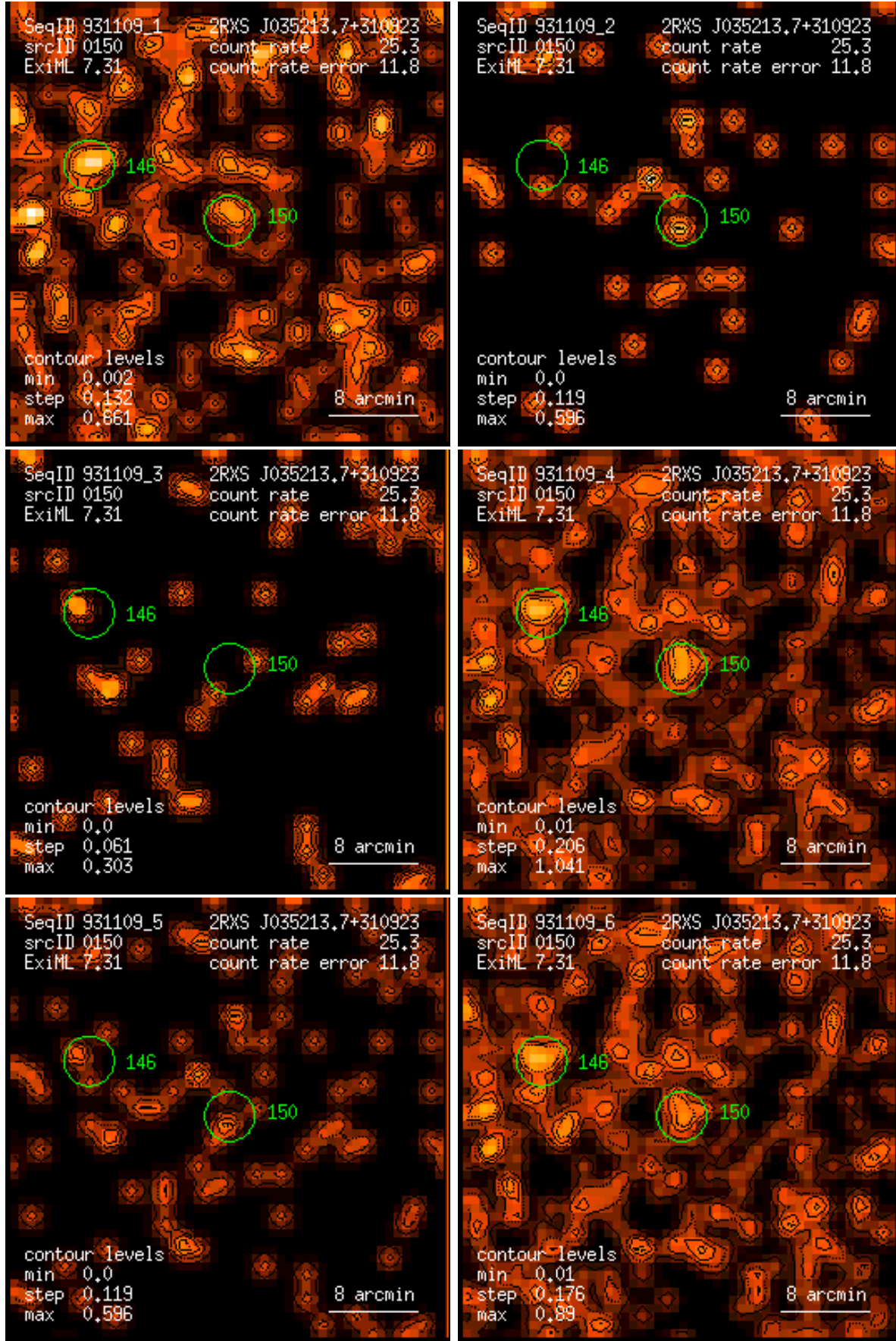
Figure 150: RASS 931109: detection 0150: band rate images, Gaussian filter: (1) PSPC channels 11 – 41, (2) 52 – 90, (3) 91 – 201, (4) 11 – 235, (5) 52 – 201, (6) 11 – 201. Broad band rates in counts/ks. Band rate contour levels in counts/ks/arcmin 2 .
