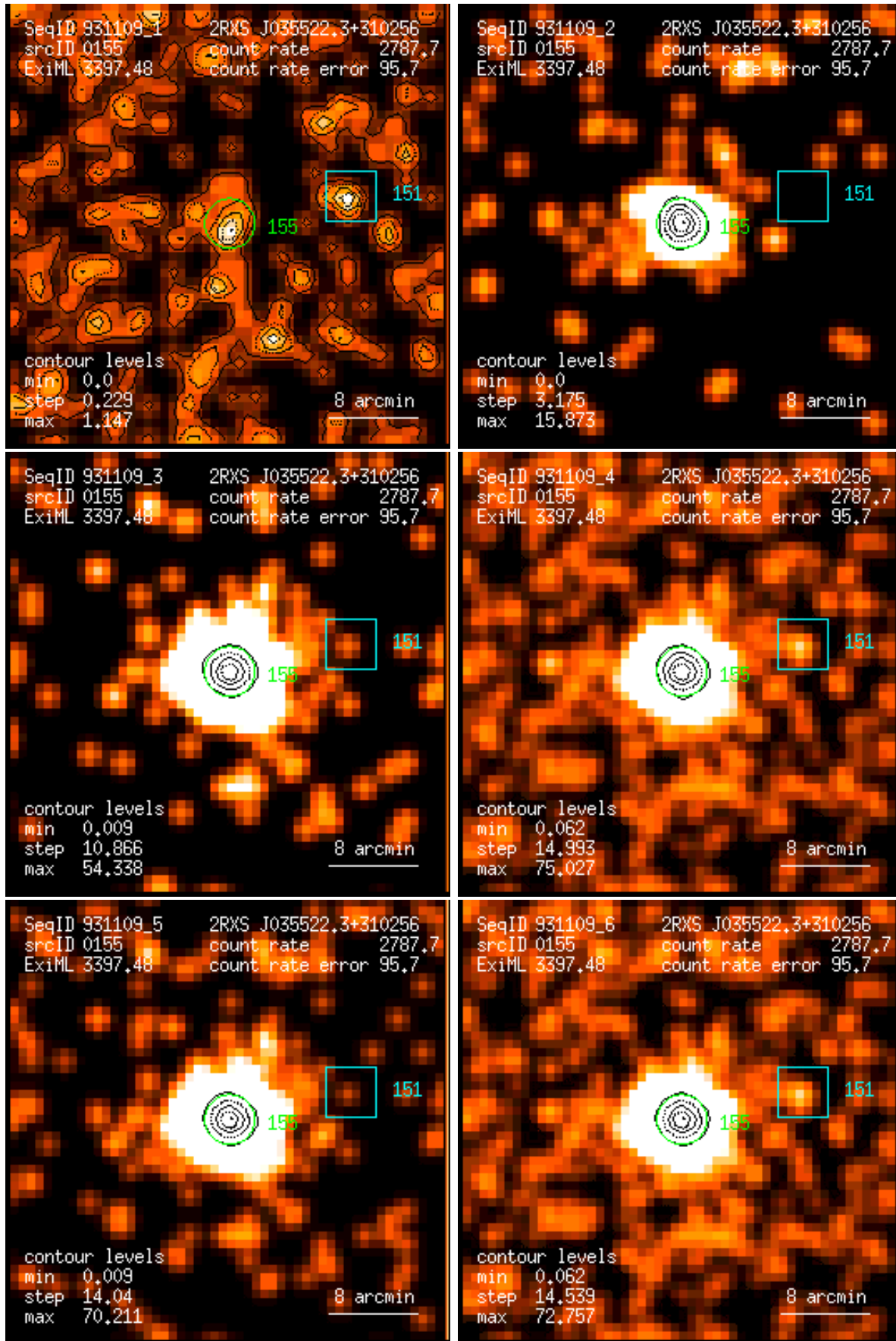
Figure 155: RASS 931109: detection 0155: band rate images, Gaussian filter: (1) PSPC channels 11 – 41, (2) 52 – 90, (3) 91 – 201, (4) 11 – 235, (5) 52 – 201, (6) 11 – 201. Broad band rates in counts/ks. Band rate contour levels in counts/ks/arcmin 2 .
