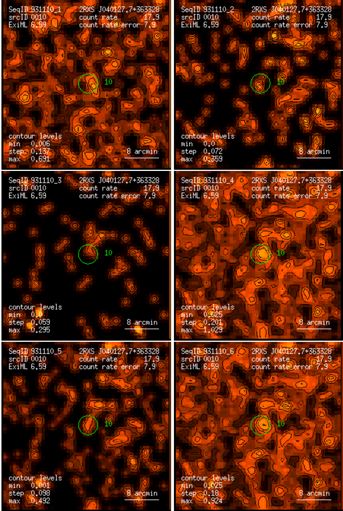
Figure 10: RASS 931110: detection 0010: band rate images, Gaussian filter: (1) PSPC channels 11 – 41, (2) 52 – 90, (3) 91 – 201, (4) 11 – 235, (5) 52 – 201, (6) 11 – 201. Broad band rates in counts/ks. Band rate contour levels in counts/ks/arcmin 2 .
