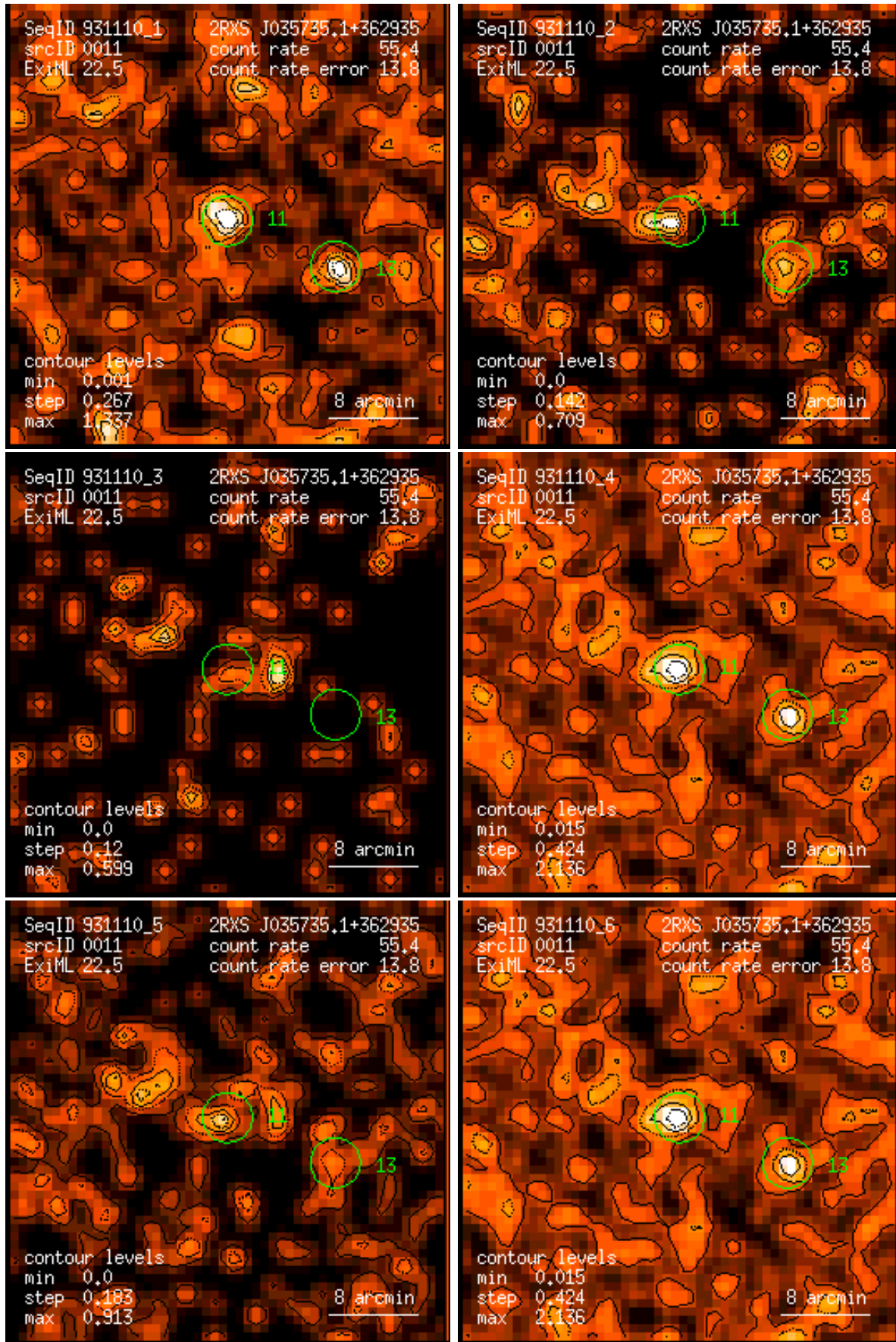
Figure 11: RASS 931110: detection 0011: band rate images, Gaussian filter: (1) PSPC channels 11 – 41, (2) 52 – 90, (3) 91 – 201, (4) 11 – 235, (5) 52 – 201, (6) 11 – 201. Broad band rates in counts/ks. Band rate contour levels in counts/ks/arcmin 2 .
