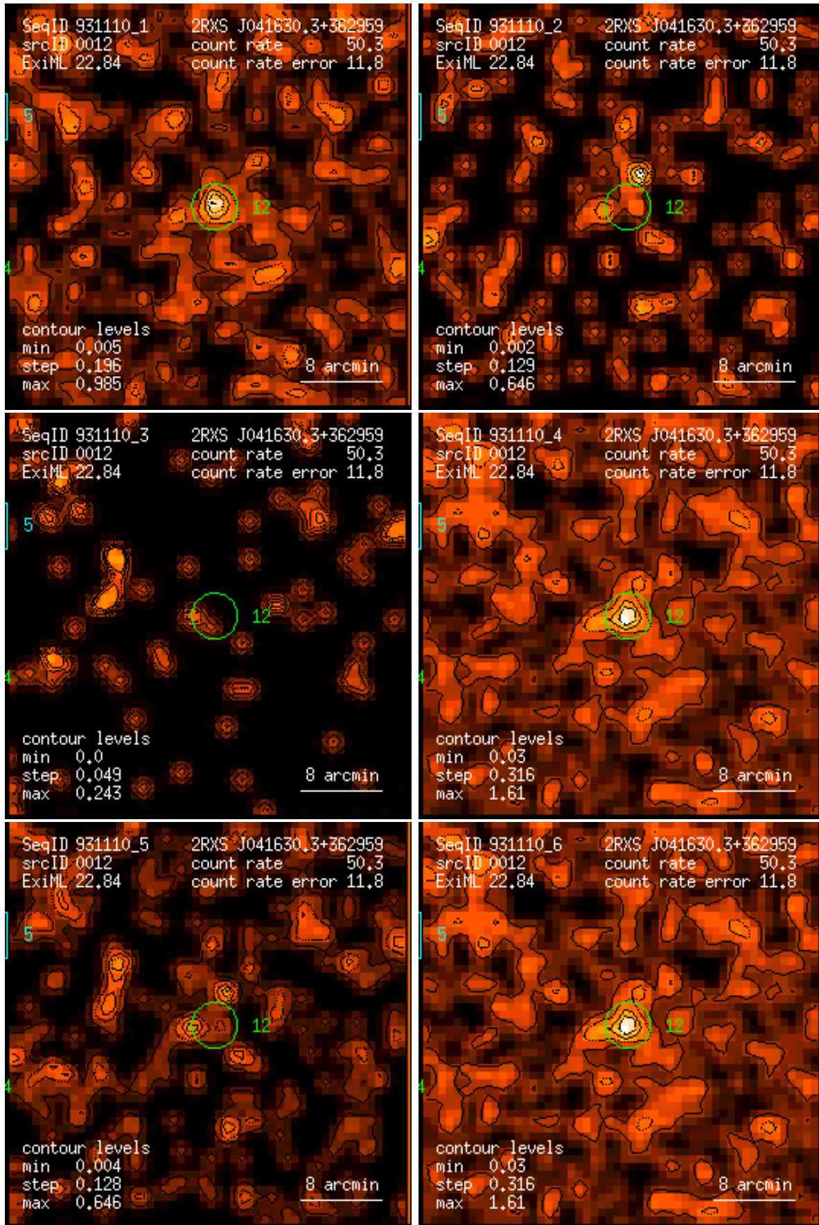
Figure 12: RASS 931110: detection 0012: band rate images, Gaussian filter: (1) PSPC channels 11 – 41, (2) 52 – 90, (3) 91 – 201, (4) 11 – 235, (5) 52 – 201, (6) 11 – 201. Broad band rates in counts/ks. Band rate contour levels in counts/ks/arcmin 2 .
