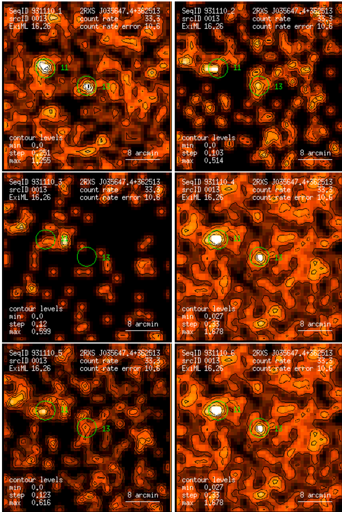
Figure 13: RASS 931110: detection 0013: band rate images, Gaussian filter: (1) PSPC channels 11 – 41, (2) 52 – 90, (3) 91 – 201, (4) 11 – 235, (5) 52 – 201, (6) 11 – 201. Broad band rates in counts/ks. Band rate contour levels in counts/ks/arcmin 2 .
