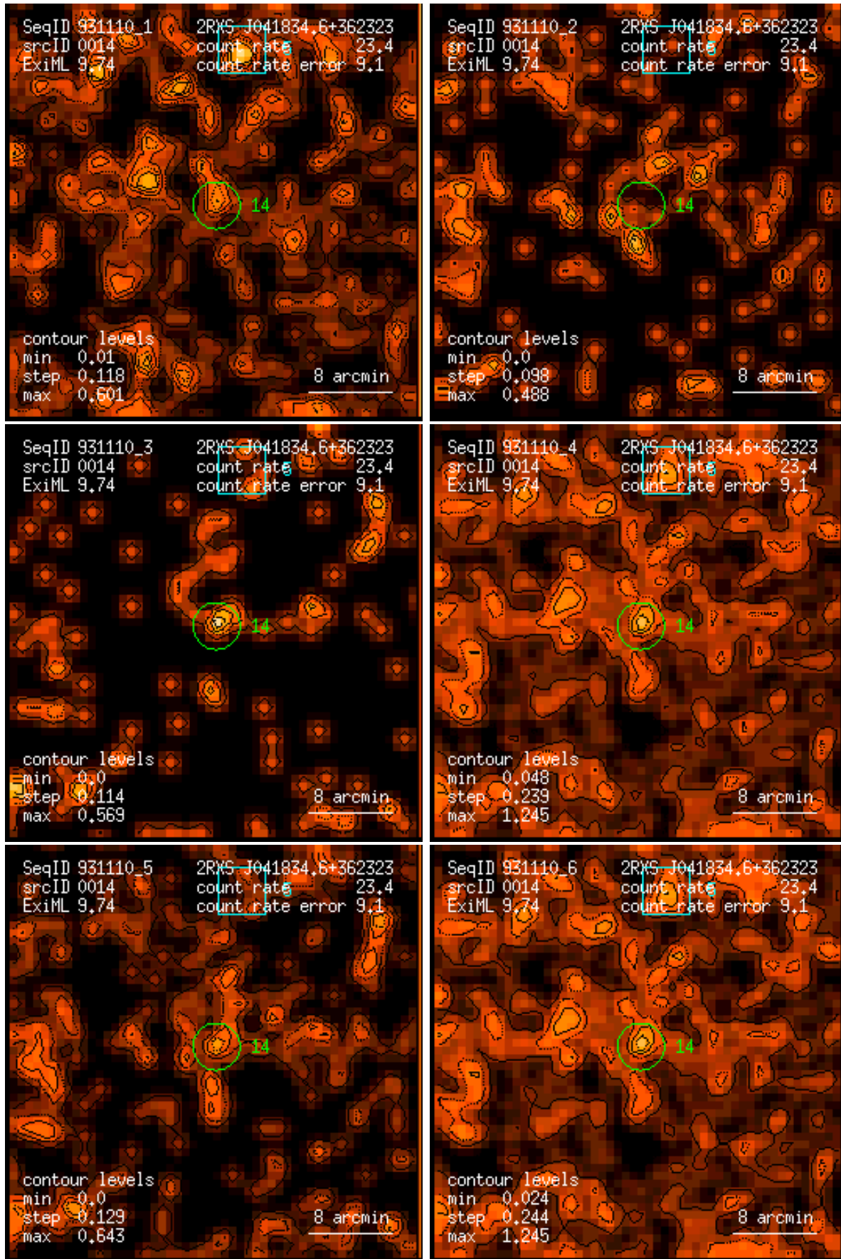
Figure 14: RASS 931110: detection 0014: band rate images, Gaussian filter: (1) PSPC channels 11 – 41, (2) 52 – 90, (3) 91 – 201, (4) 11 – 235, (5) 52 – 201, (6) 11 – 201. Broad band rates in counts/ks. Band rate contour levels in counts/ks/arcmin 2 .
